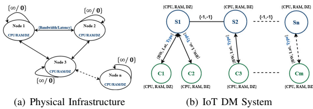
Fig. 3: Input Graph Models
