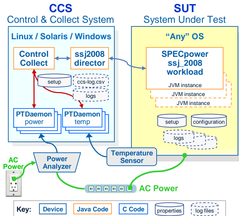
Figure 1 – Block Diagram
