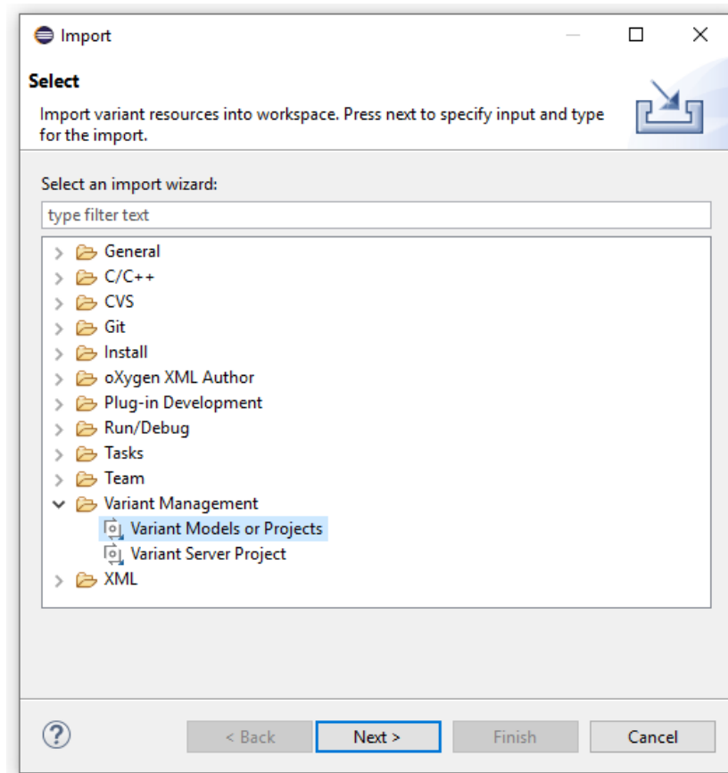
Figure 6.65. Import Dialog
