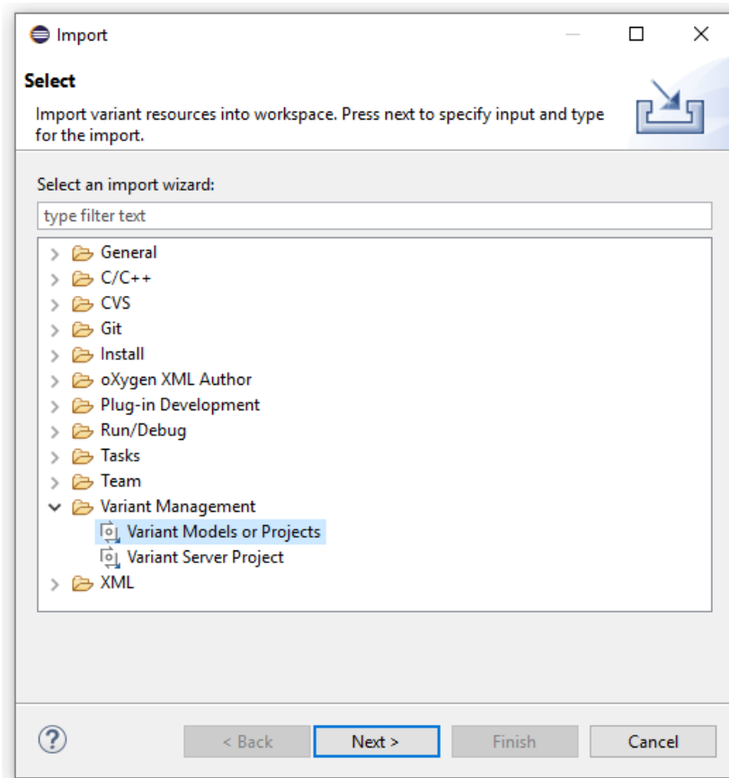
Figure 6.59. Import Dialog
