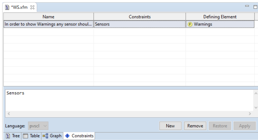
Figure 7.3. Constraints view
