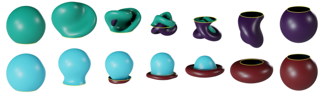
Fig. 29. Inversion of cut-open sphere. Top: Discrete geodesic interpolation without repulsion (green to purple). Bottom: Geodesic interpolation with repulsion (blue to red). The fixed surface boundary is shown as yellow curve.
