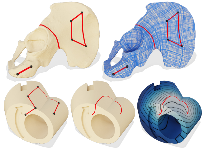
Fig. 26. An intrinsic triangulation conforming to geodesic or Bézier curves can be used to directly enforce boundary conditions for PDE-based algorithms. Here we compute the smoothest cross field aligned to a set of geodesic paths ( top ), and solve a Poisson equation with Dirichlet boundary conditions enforced along a geodesic Bézier curve ( bottom ).
