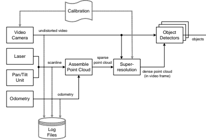
Fig. 1. Our robotic platform, hardware specifications, and data flow: a sparse point cloud is reconstructed in software by knowing the relative pose between the pan/tilt unit and the video camera, and correcting for robot motion using odometry. The depth of every pixel is then inferred, and features from the 2-d image and the 3-d point cloud are combined by our probabilistic object detectors.
