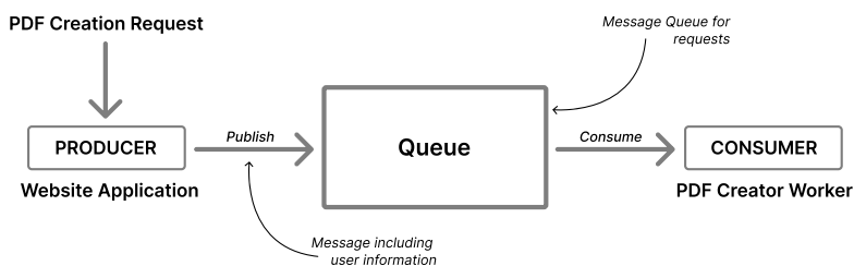
Figure F.1. PDF File Creation Example
