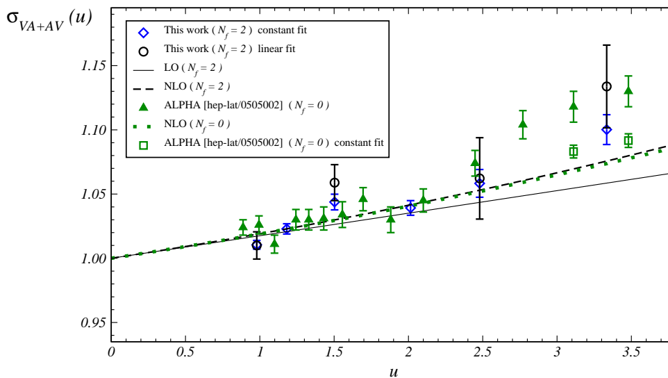
Figure 2: The step scaling function \sigma_{VA+AV}(u) (discrete points) is compared to the LO and NLO perturbative results. In order to evaluate the quality of our data we compare our N_f = 2 results with quenched data from ref. [8]. Results are preliminary.
