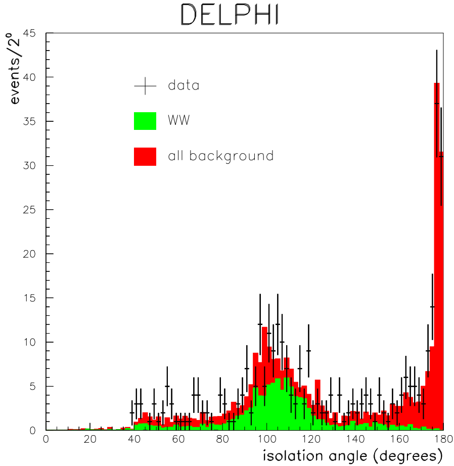
Figure 9: Isolation angle of selected electrons, muons and single charged particle tracks in the sample selected to mimic the background to the selected q\bar{q}\nu\bar{\nu} sample. The points are the data, summed over all energy points, the light (green) histogram is the predicted WW contribution, and the dark (red) histogram is the rest of the background.
