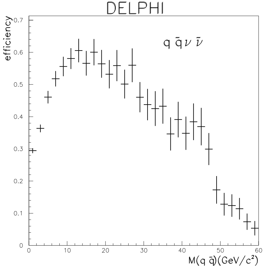
Figure 7: Combined selection efficiency of the q\bar{q}\nu\bar{\nu} analysis, averaged over all energy points, as a function of the generated M(q\bar{q}) mass.
