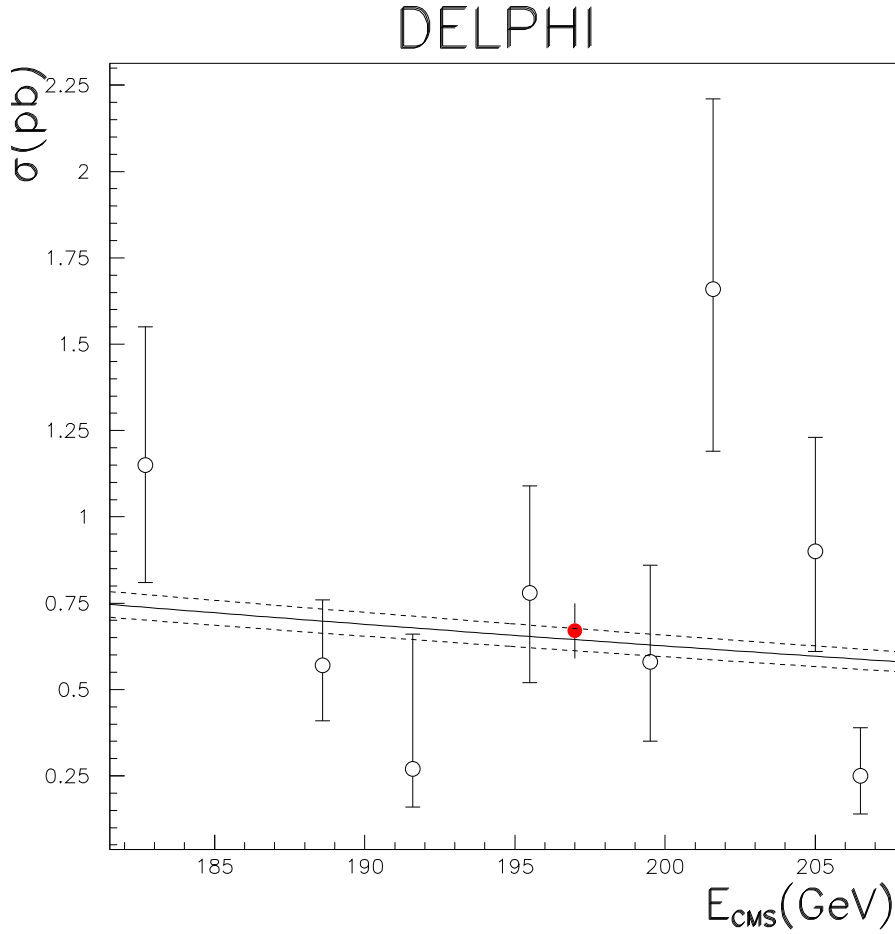
Figure 13: Combined Z\gamma^* cross-section as a function of the centre-of-mass energy, using the Matrix Element signal definition (see section 2). The solid line is the Standard Model prediction; the dashed line represents a 5% uncertainty around this prediction. The full (red) point is the average cross-section result, plotted at the luminosity-weighted average centre-of-mass energy.
