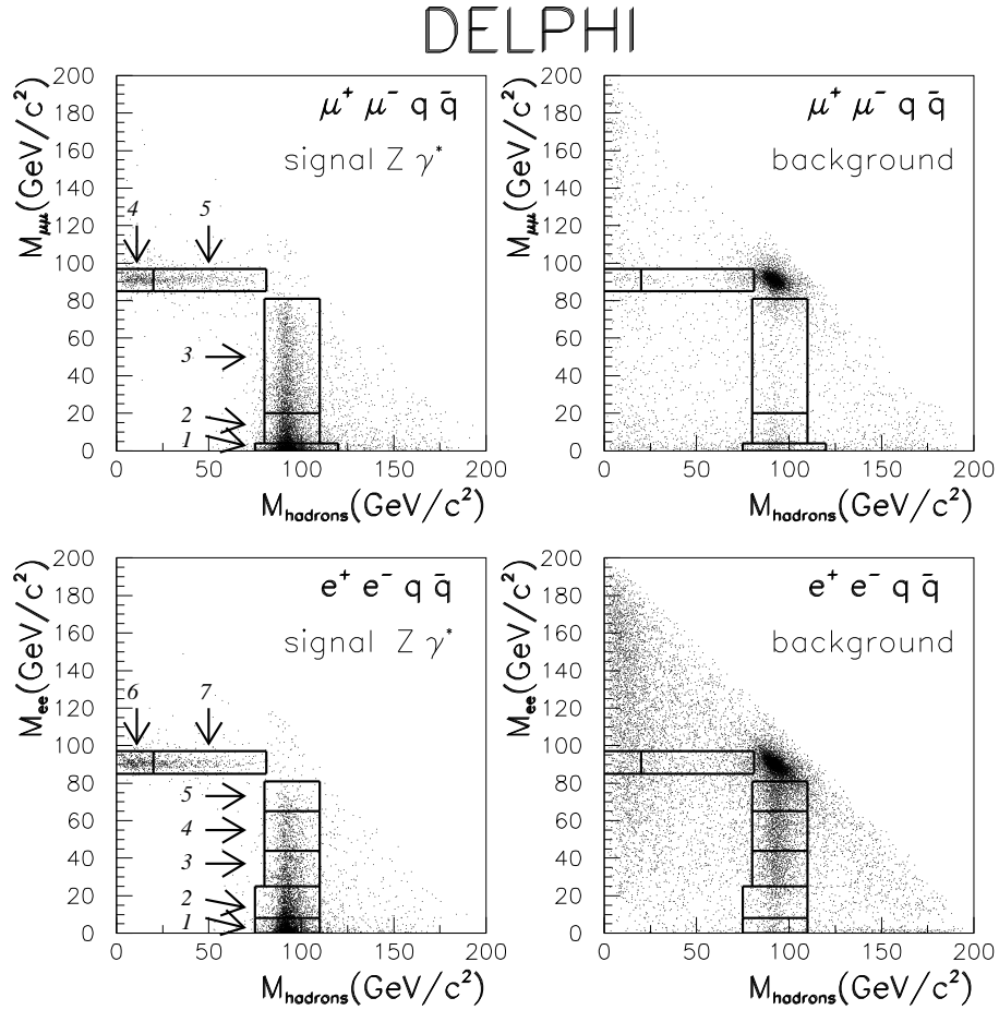
Figure 4: l^+l^-q\bar{q} final state: Bidimensional distributions in the plane of the di-fermion masses predicted by the Standard Model for signal Z\gamma^* (left-hand plots) and background (right-hand plots) for the two channels studied, averaged over all energy points. The bins used for the fit are also shown.
