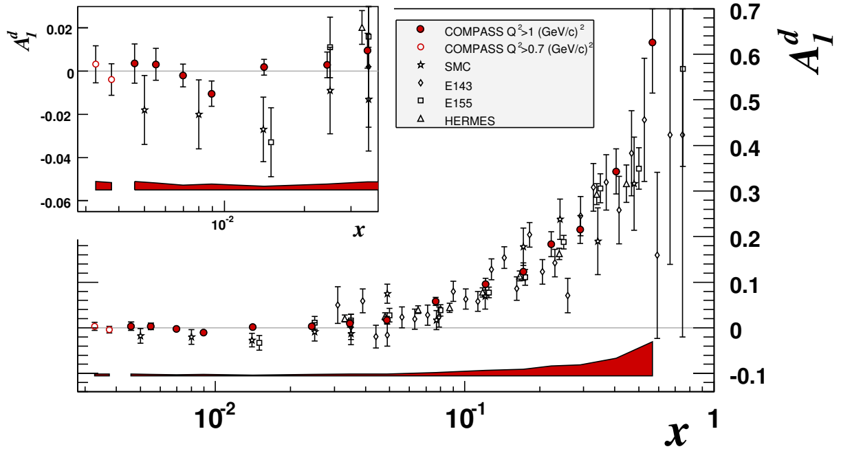
Figure 3: The asymmetry A_1^d(x) as measured in COMPASS and previous results from SMC [5], HERMES [4], SLAC E143 [2] and E155 [3] at Q^2 > 1 (GeV/c) ^2 . The SLAC values of g_1/F_1 have been converted to A_1 and the E155 data corresponding to the same x have been averaged over Q^2 . Only statistical errors are shown with the data points. The shaded areas show the size of the COMPASS systematic errors.
