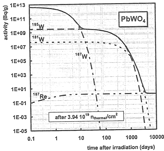
Fig. 1. Calculated induced activity of the \text{PbWO}_4 sample irradiated.
