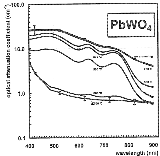
Fig. 2. Optical attenuation coefficient of the irradiated sample before annealing and after successive annealing temperatures.
