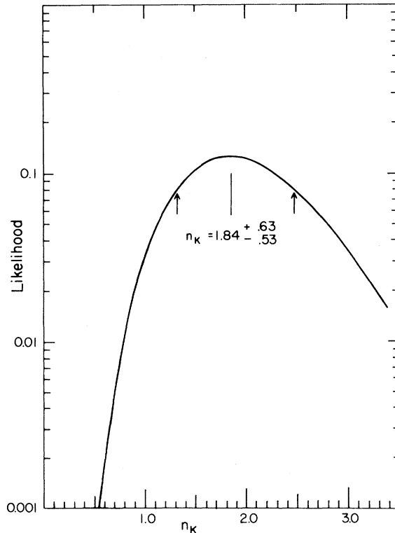
FIG. 2. Multiplicity likelihood distribution for observed K^0 .
