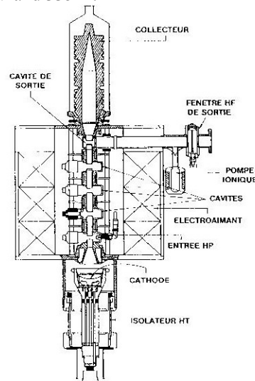
Figure 5 A TH2100C klystron (cut through view)
