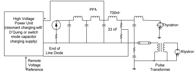
Figure1. Modulator basic circuit diagram
