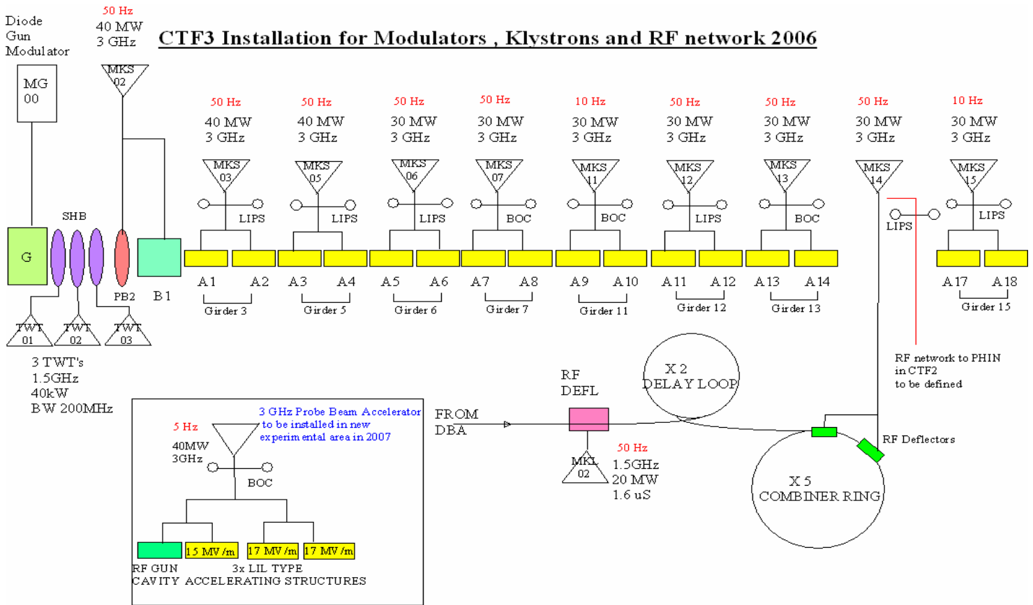
Figure 6 Installation for modulators, klystrons and RF network
