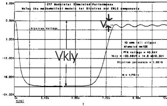
Figure 3 Klystron Voltage Simulation
