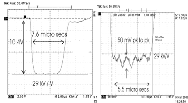
Figure2. Klystron Waveform and ripple on flat top (+/- 0.25%)
