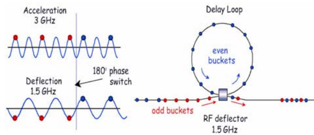
Figure 8 Phase coding of RF bunches
