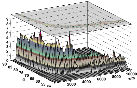
Figure 3: Maximum relative density of lost particles per cavity and mm^2 collected from 500 different configurations of misalignment.
