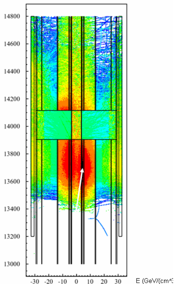
Figure 2: Energy deposition per ion (500 simulated) in a thick horizontal slice through the magnet in Figure 1. The white arrow indicates the impact on the beam pipe in the dipole, downstream of which a drift space and quadrupole can be seen. In the dipole, the correct field map was implemented inside the cold mass. It was sufficient to model the quadrupole as a copy of the dipole magnet but without magnetic field.
