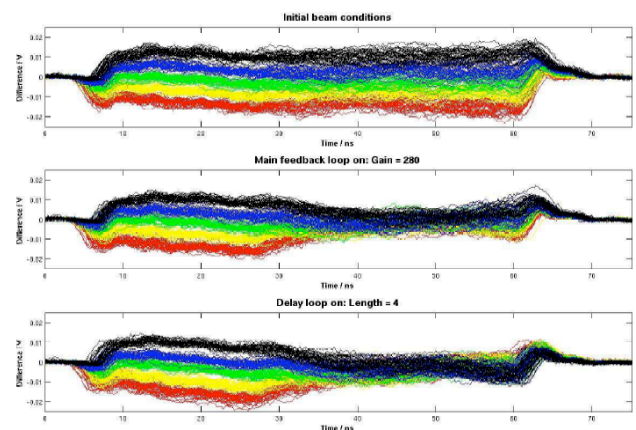
Figure 7: Beam position (arbitrary units) vs. time in nanoseconds. The bunchtrain starts at c. 6ns and ends at c. 62ns. 40 sequential beam pulses per position setting are shown.
