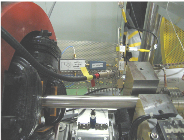
Figure 3: Downstream section of the ATF beamline showing the BPM signal processor.
