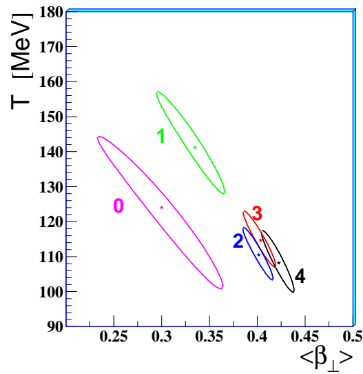
Figure 10. The 1 \sigma confidence level contours from fits in each centrality class.
