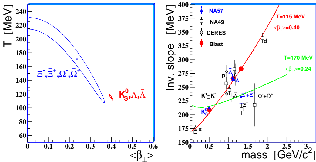
Figure 9. Left: the thermal freeze-out temperature versus the average transverse flow velocity for blast-wave fits using a linear ( n = 1 ) velocity profile. The 1 \sigma contours are shown, with the markers indicating the optimal fit locations. Right: prediction of the blast-wave model for inverse slopes (see text for details).
