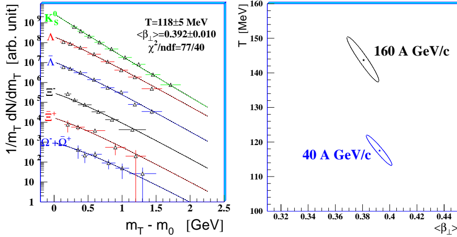
Figure 8. Left: blast-wave fits to the transverse mass spectra of strange particles for the most central 53% of the Pb{Pb inelastic cross-section at 40 A GeV/c.
