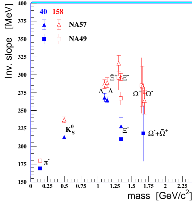
Figure 6. Apparent temperature as a function of the particle rest mass in Pb{Pb at 40 A GeV /c (closed symbols, in blue on-line) as compared to 158 A GeV /c (open symbols, in red). NA 49 results for negative pions [8] and multi-strange hyperons [24, 22, 25] are also shown (squares). For display purpose the ordinate scale has been zero-suppressed.
