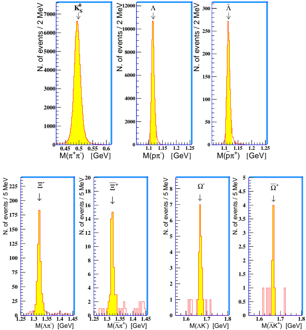
Figure 2. Sample invariant mass spectra for \Xi^+ , \Xi^- , \Omega^- , and \bar{\Omega}^+ . The arrows show the PDG mass values [17].
