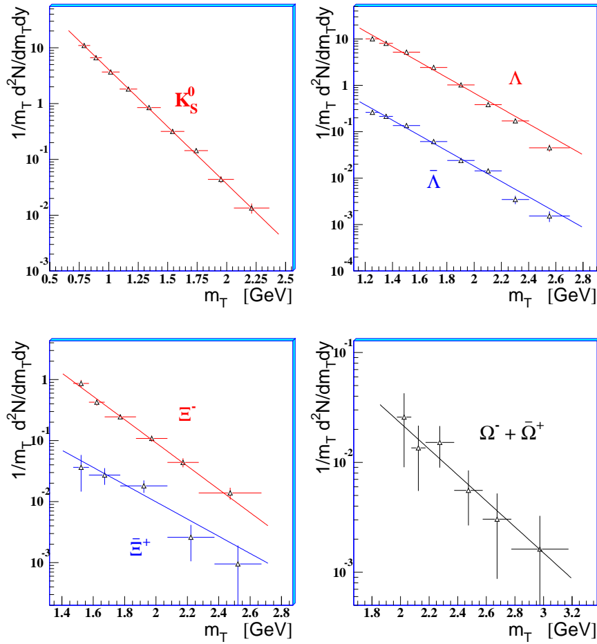
Figure 5. Transverse mass spectra of strange particles for the most central 53% of the Pb{Pb inelastic cross-section. The superimposed exponential functions have inverse slopes equal to the T_{app} values obtained from the maximum likelihood fits.
