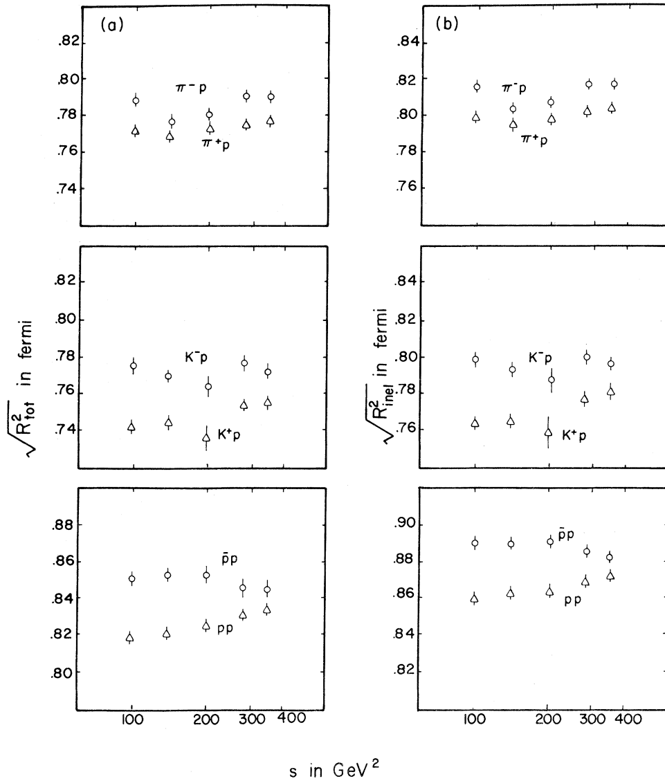
FIG. 6. The rms interaction distances for (a) the total and (b) the inelastic cross sections as a function of s for \pi^\pm p , K^\pm p , pp , and \bar{p}p . The errors are calculated as for Fig. 3.
