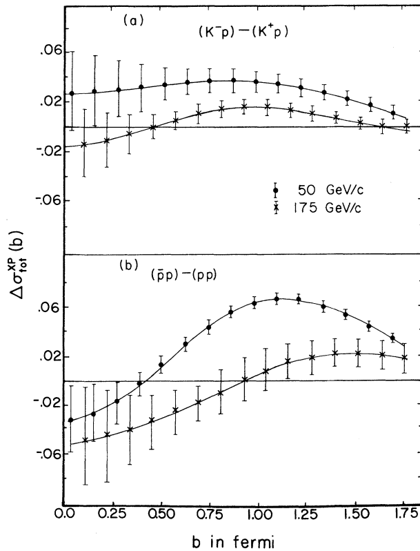
FIG. 10. \Delta\sigma_{\text{tot}}^{xp}(b) for (a) Kp and (b) pp at P=50 GeV/c (●) and at P=175 GeV/c (×).
