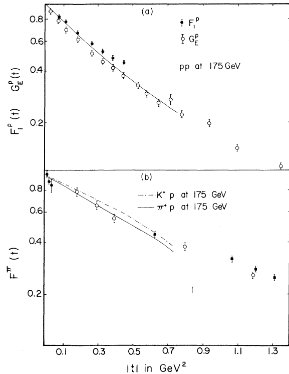
FIG. 11. (a) F_1^p(t) (●) and G_E^p(t) (○) proton form factors from Ref. 18. The solid line corresponds to the calculated \langle D_p(b) \rangle using Eq. (14) for pp scattering 175 GeV/c, normalized to \langle D_p(b) \rangle = 1 , at t=0 . (b) Pion form factor measurements from Ref. 19 (●) and Ref. 20 (○, ■). In the region of this measurement, the solid (dotted) line corresponds to the Fourier transform of the pion (Kaon) hadronic density calculated using (14) for \pi^+p ( K^+p ) and \pi^0p scattering at 175 GeV/c, normalized to \langle D_\pi(b) \rangle = 1 [ \langle D_K(b) \rangle = 1 ], at t=0 .
