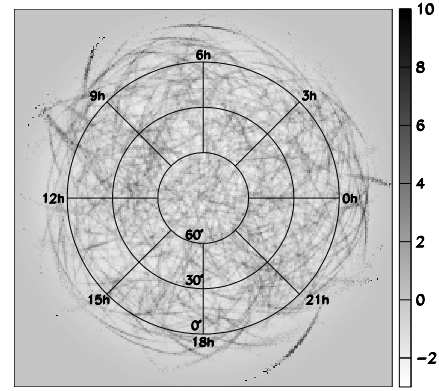
Figure 2. \chi_1 (Equation 1) distribution for the HiRes-I monocular data set.
