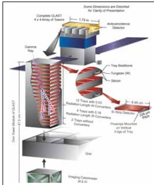
Figure2 Schematic of LAT
