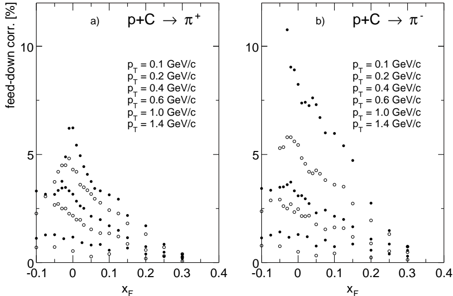
Figure 13: Feed-down correction to pion from weak decays for a) \pi^+ and b) \pi^-
