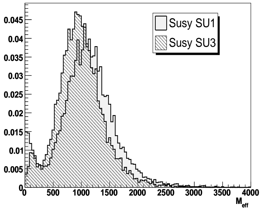
Figure 2: The discriminator M_{eff} (defined in table 3) for the SU1 and SU3 benchmark models
