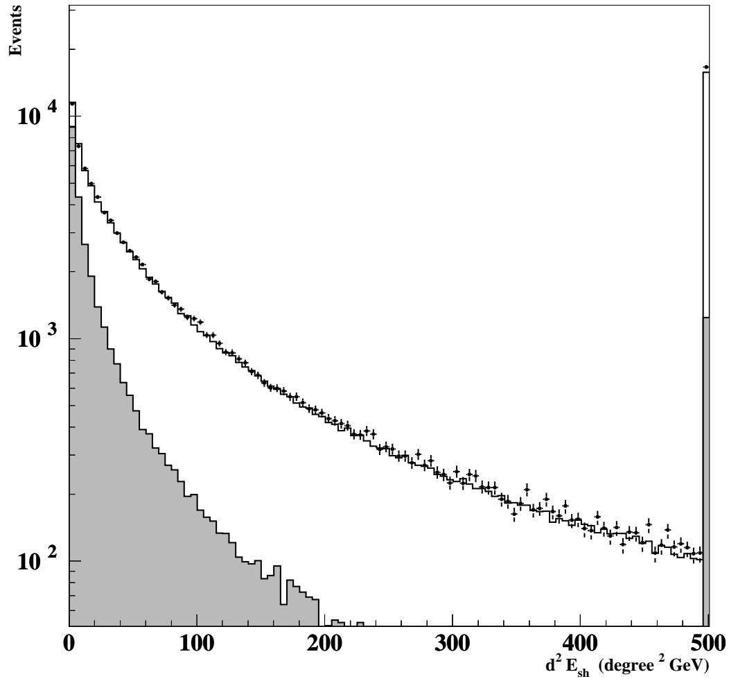
Figure 8: Distributions of the quantity d_{sh-ch}^2 E_{sh} used for rejection of hadronic showers in the HPC for the inclusive \tau sample of photons with all identification requirements applied except the cut on this variable. Data are shown as dots and simulation by a solid line. The shaded area shows the contribution from showers induced by charged hadrons. The last bin shows the overflows.
