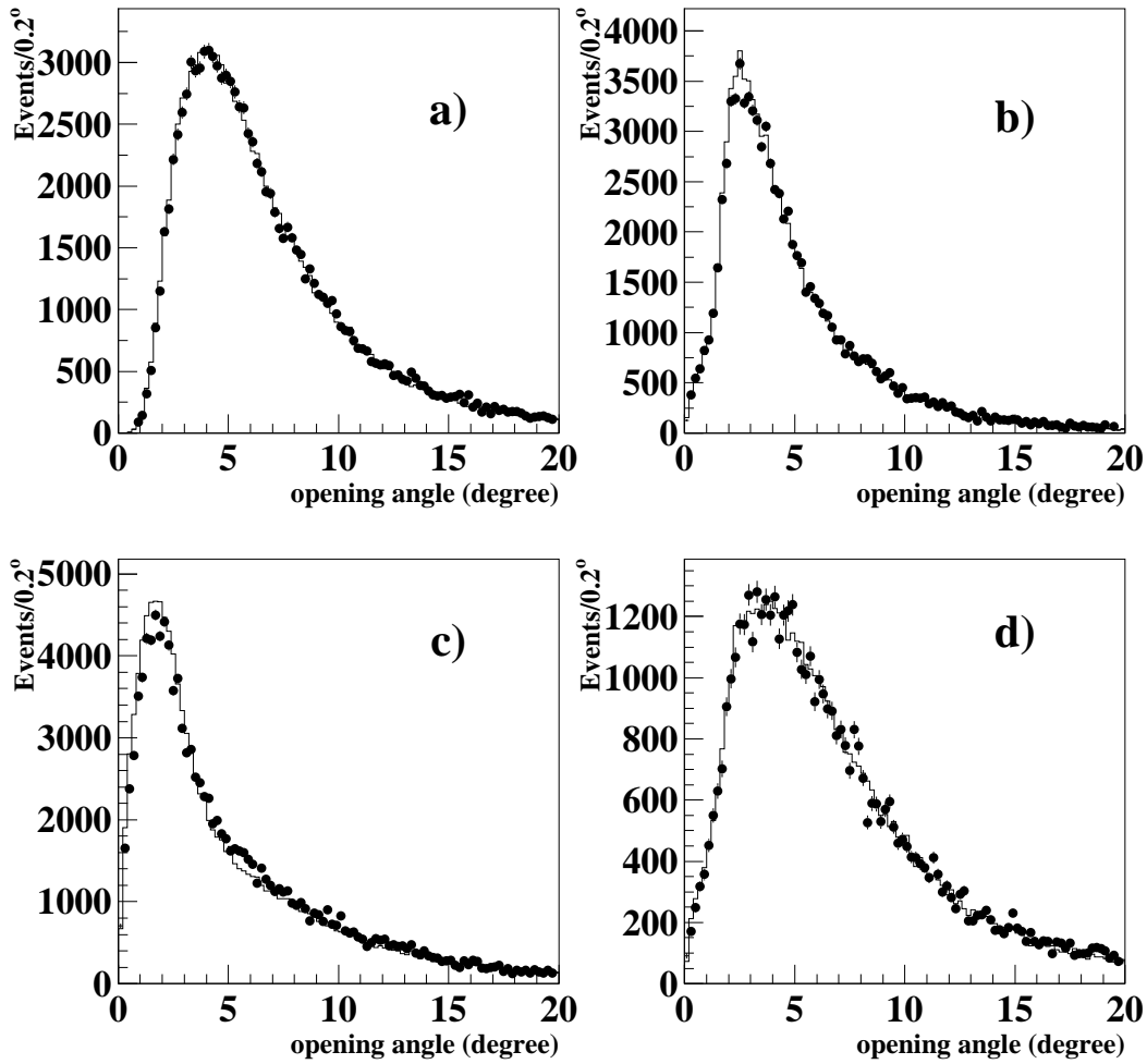
Figure 10: Distribution of opening angle between different types of showers: a) a neutral shower fulfilling the \gamma identification with a shower associated to a track b) two neutral showers fulfilling the \gamma identification, c) a neutral shower failing the \gamma identification with a shower associated to a track c) a neutral shower fulfilling the \gamma identification with another one failing it. Data are shown as dots and simulation by a solid line.
