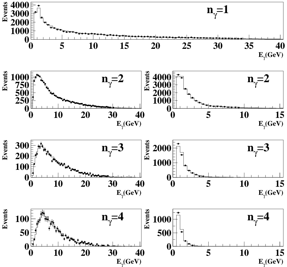
Figure 9: Energy distributions of identified photons in the HPC for \tau -decays containing 1, 2, 3 or 4 such clusters. The figures on the left represent the most energetic cluster in the decay and those on the right the least energetic. Data are shown as dots and simulation by a solid line.
