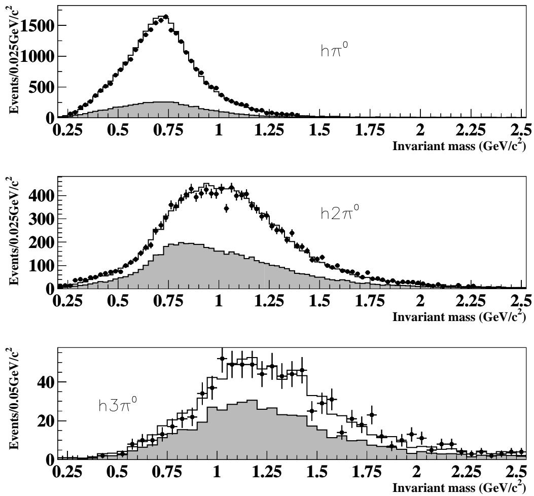
Figure 17: Invariant-mass distributions for the one-prong decays selected with the neural network. Data are shown as dots, simulation by a solid line. The shaded area shows the background prediction from simulation.
