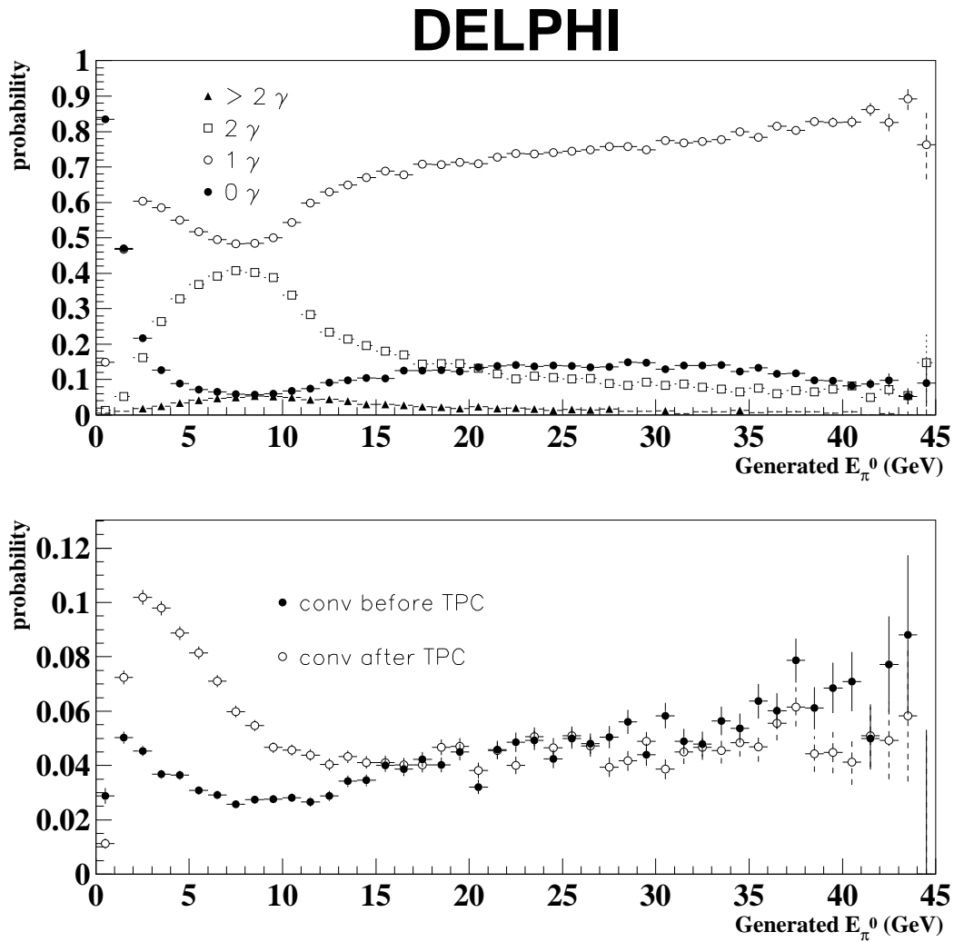
Figure 11: The fraction events, as a function of \pi^0 energy with: (top) 0,1,2, or more than 2, photons reconstructed; (bottom) a reconstructed conversion before or after the TPC, for a sample of simulated non-radiative \rho -decays.
