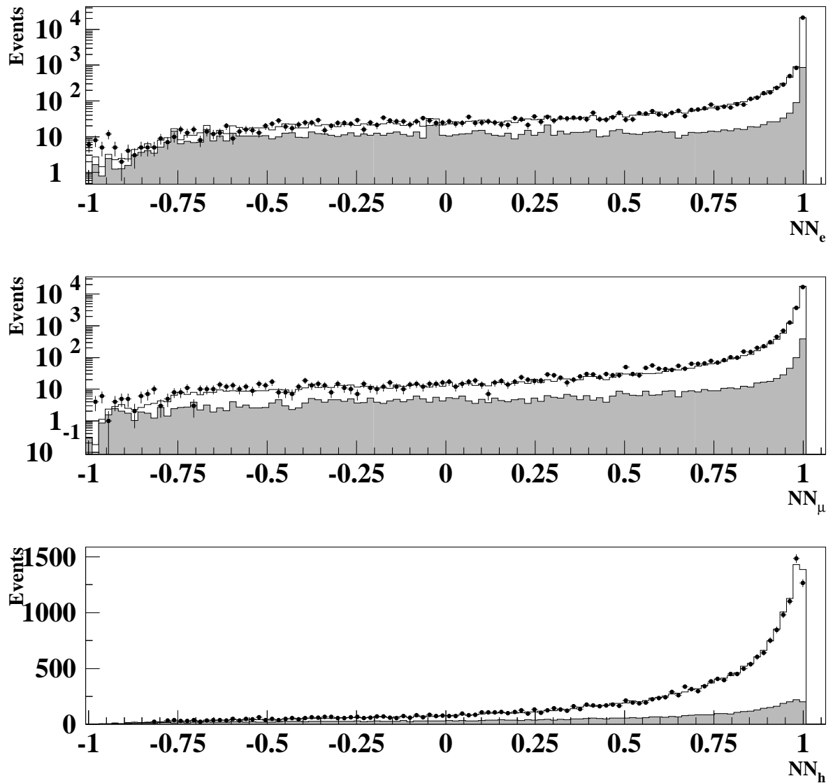
Figure 15: Maximum-output neuron value in one-prong analyses. For each event the output of the class whose output neuron is maximum is represented. Data are shown as dots and simulation by a solid line. The shaded area represents the background events.
