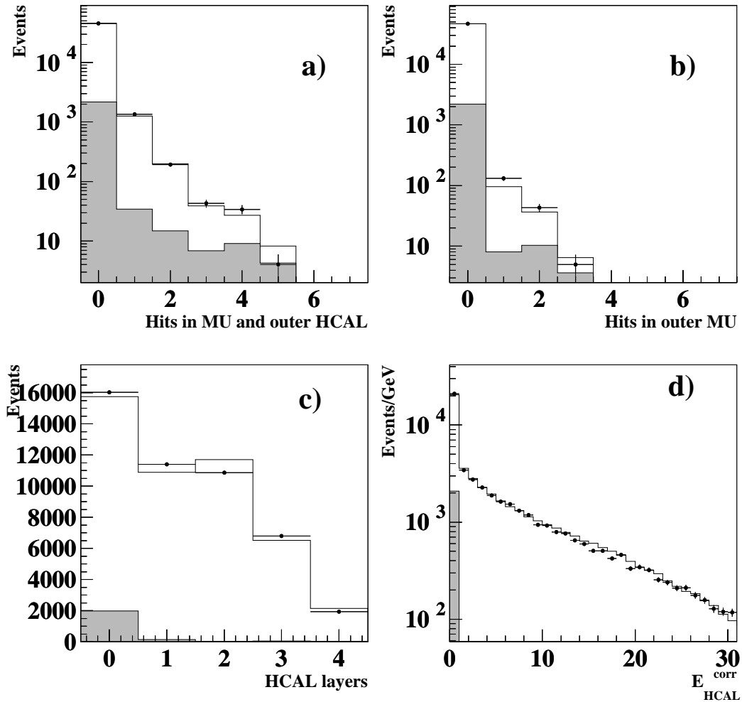
Figure 4: Muon-identification variables for hadron test samples in \tau -decays: a) number of muon chamber hits including the outer HCAL layer; b) number of muon chamber hits in the outer muon chambers; c) number of layers in the HCAL; d) corrected deposited energy in the HCAL. Data are shown as dots and simulation after the corrections described in the text, by a solid line. The shaded area represents the non-hadron background.
