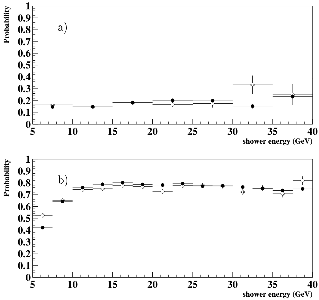
Figure 6: \pi^0 -identification probability in a single shower as a function of the shower energy, obtained from isolated- \gamma samples (a) and \pi^0 sample in tightly-tagged \rho decays (b). Data are represented by crosses and simulation by filled circles.
