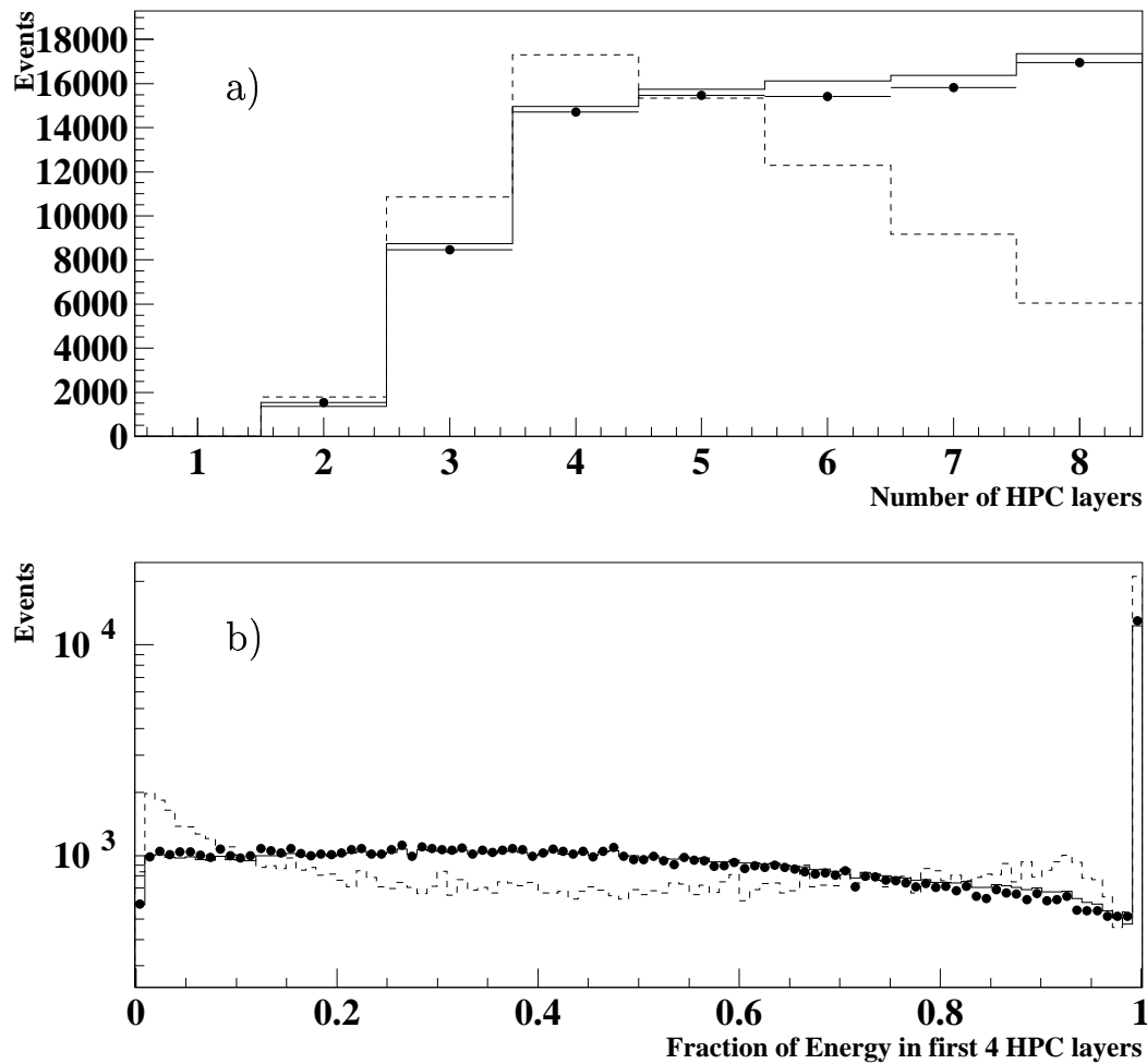
Figure 7: Distribution for candidate photon clusters for the inclusive sample of \tau -decays: Number of HPC layers hit (a); fraction of energy deposited in the four innermost layers (b). Data are shown as dots and simulation by a solid line. The dashed line shows in arbitrary normalization the distributions for showers produced from charged hadrons.
