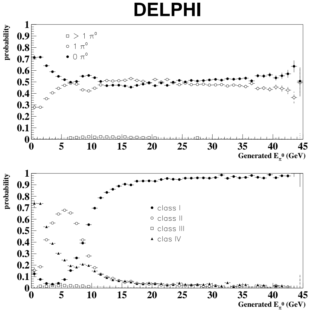
Figure 13: Total \pi^0 reconstruction efficiency (top) and probability to reconstruct a \pi^0 in any of the classes described in the text (bottom) as a function of the \pi^0 energy for simulated \rho decays.
