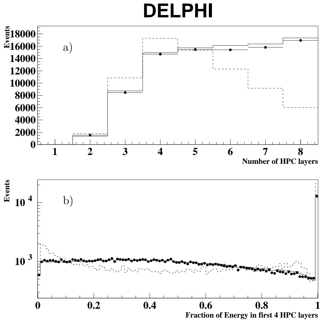
Figure 7: Distribution for candidate photon clusters for the inclusive sample of \tau -decays: Number of HPC layers hit (a); fraction of energy deposited in the four innermost layers (b). Data are shown as dots and simulation by a solid line. The dashed line shows in arbitrary normalization the distributions for showers produced from charged hadrons.
