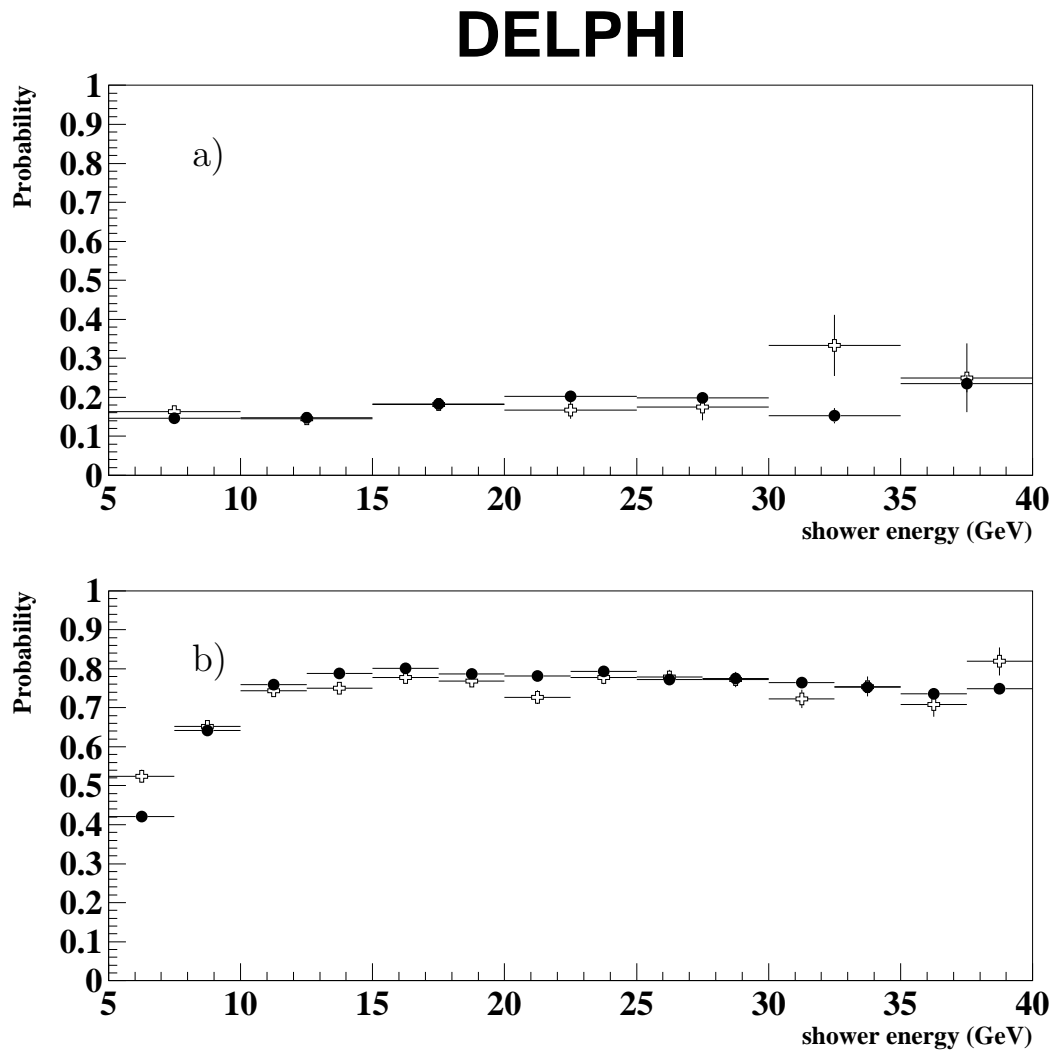
Figure 6: \pi^0 -identification probability in a single shower as a function of the shower energy, obtained from isolated- \gamma samples (a) and \pi^0 sample in tightly-tagged \rho decays (b). Data are represented by crosses and simulation by filled circles.
