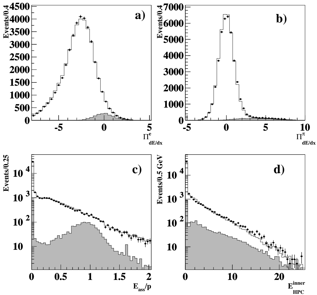
Figure 2: Distributions for hadron test samples in \tau -decays of electron-hadron separation variables: a) the variable \Pi^c_{dE/dx} ; b) the variable \Pi^\pi_{dE/dx} ; c) the variable \frac{E_{ass}}{p} ; d) the energy deposited in the innermost four layers of the HPC. Data are shown as dots and simulation by a solid line. The shaded region represents the simulated background including other \tau -decays.
