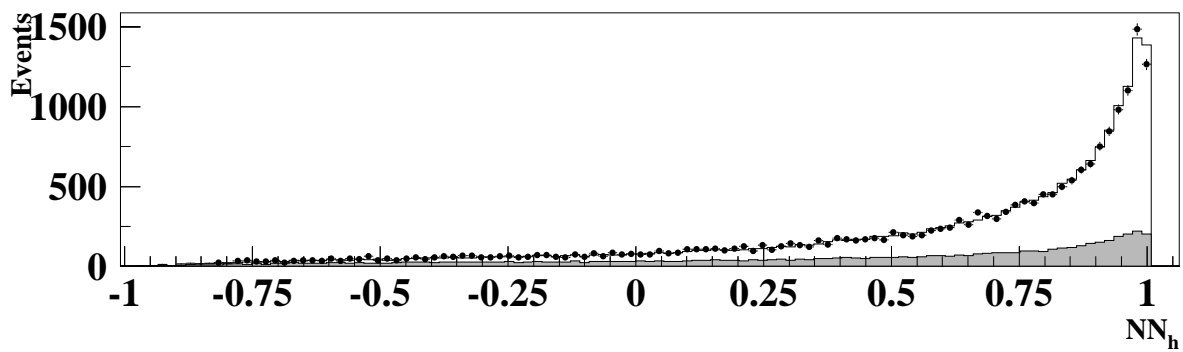
Figure 15: Maximum-output neuron value in one-prong analyses. For each event the output of the class whose output neuron is maximum is represented. Data are shown as dots and simulation by a solid line. The shaded area represents the background events.
