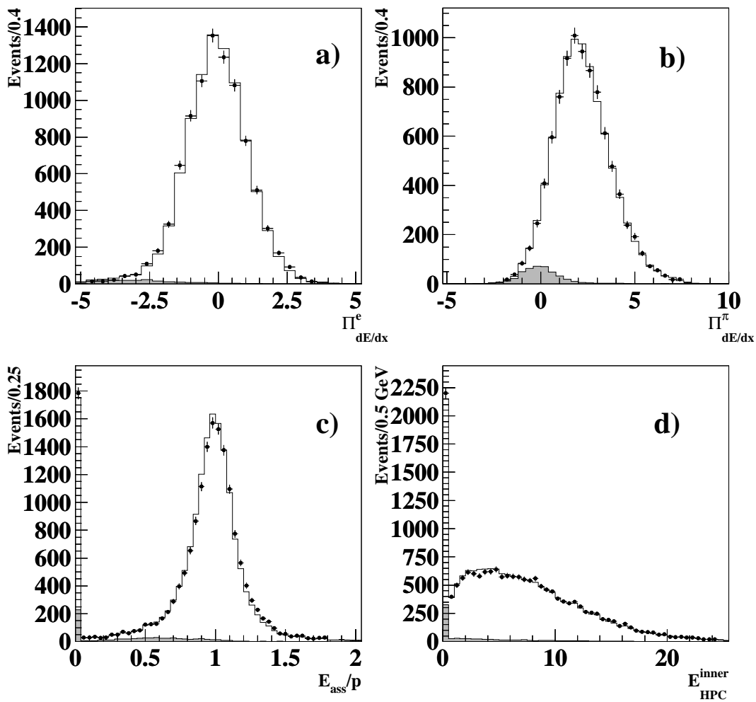
Figure 1: Distributions for electron test samples in \tau -decays : a) the variable \Pi^e_{dE/dx} ; b) the variable \Pi^\pi_{dE/dx} ; c) the variable \frac{E_{ass}}{p} ; d) the energy deposited in the innermost four layers of the HPC. Data are shown as dots and simulation by a solid line. The shaded region represents the simulated background including other \tau -decays.
