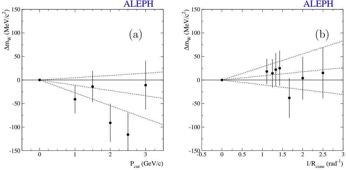
Figure 5: \Delta m_W versus (a) PCUT in GeV/c and (b) inverse CONE radius (R) in rad -1 for q\bar{q}q\bar{q} data. The dashed lines denote the fitted slopes and \pm 1\sigma errors. The correlation with respect to the standard analysis is taken into account in the error on the mass difference for each reconstruction.
