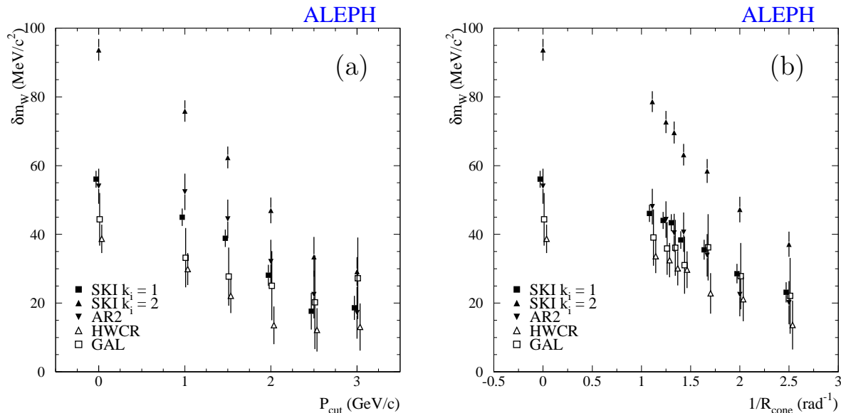
Figure 4: \delta m_W versus (a) PCUT in GeV/ c and (b) inverse CONE radius (R) in \text{rad}^{-1} for SKI (2 k_i values), AR2, HWCR and GAL models in the q\bar{q}q\bar{q} channel.
