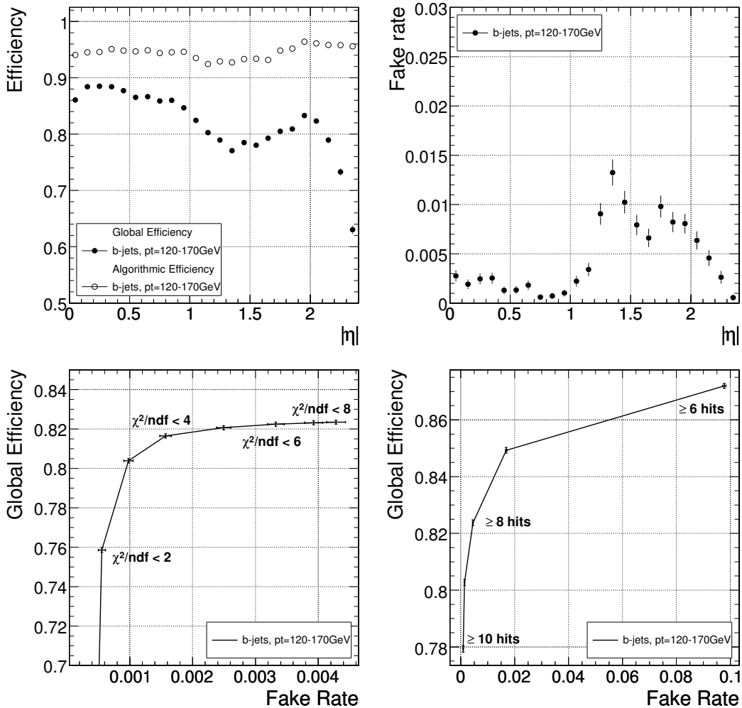
Figure 16: Global track reconstruction efficiency for b jets with transverse momenta between 120 and 170 GeV/ c , including low luminosity pileup. Upper row: efficiency (left) and fake rate (right). Lower row: evolution of the average efficiency and fake rate for different cuts on the normalised \chi^2 of the track (left) and for different number of hits used (right).
