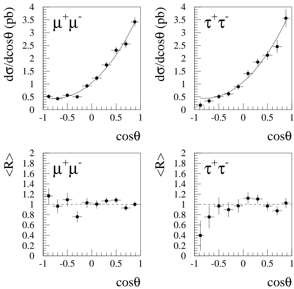
Figure 12: Bin-by-bin averages, \langle R \rangle , for \mu^+\mu^- and \tau^+\tau^- final states. The lower plots show the values of \langle R \rangle while the upper plots show the SM d\sigma/d\cos\theta multiplied by \langle R \rangle at the luminosity weighted centre-of-mass energy for each measurement channel.
