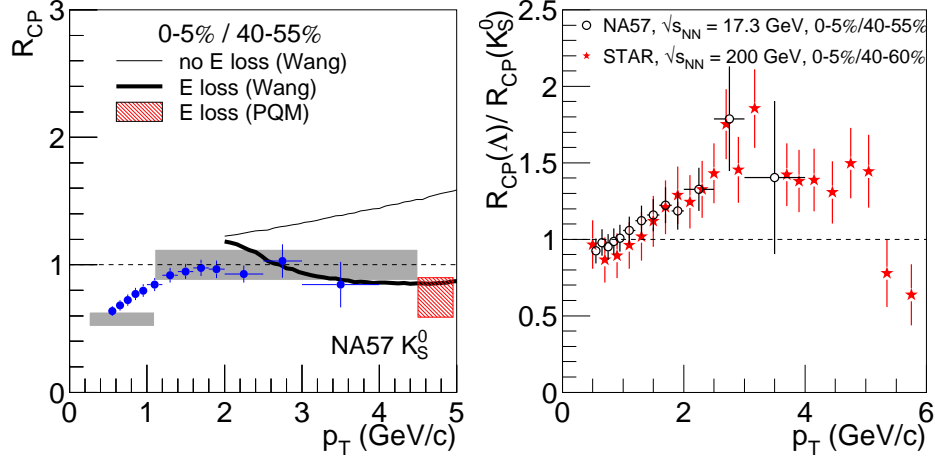
Fig. 2. Left: K_S^0 R_{CP}(p_T) compared to predictions [ 13, 14] with and without energy loss. Right: ratio of \Lambda R_{CP} to K_S^0 R_{CP} , as a function of p_T , at the SPS (NA57 at \sqrt{s_{NN}} = 17.3 GeV) and at RHIC (STAR at \sqrt{s_{NN}} = 200 GeV [ 1, 15]).
