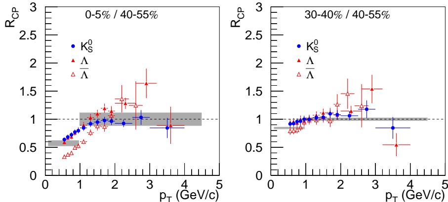
Fig. 1. R_{CP} ratios for singly-strange particles in Pb–Pb collisions at \sqrt{s_{NN}} = 17.3 GeV [ 9]. The error bars show the quadratic sum of the statistical errors and the p_T -dependent systematic errors ( < 7\% ). Shaded bands centered at R_{CP} = 1 represent the systematic error due to the uncertainty in the ratio of the values of \langle N_{coll} \rangle in each class; shaded bands at low p_T represent the values expected for scaling with the number of participants, together with their systematic error.
