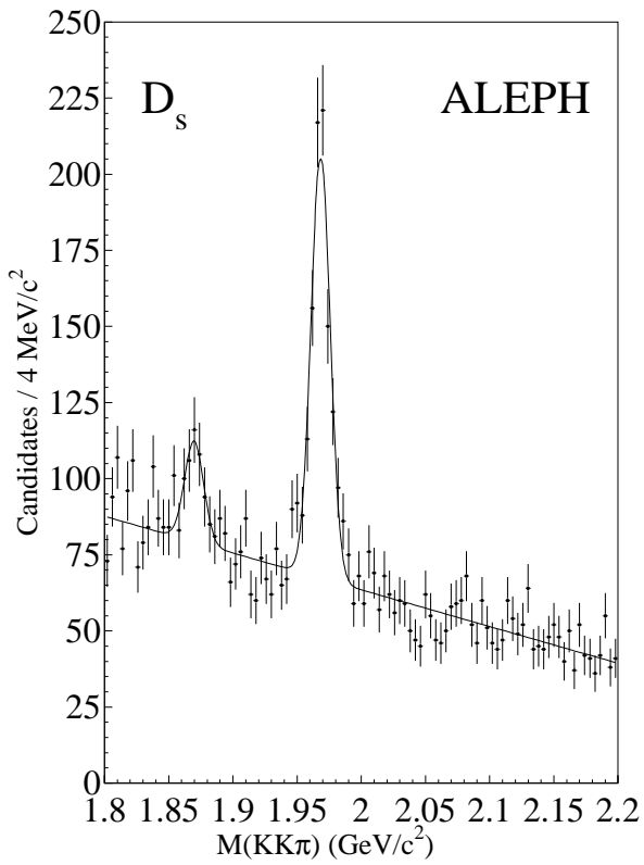
Figure 5.7: Mass spectra for D^0 \rightarrow K^- \pi^+ , D^+ \rightarrow K^- \pi^+ \pi^+ , D_s \rightarrow K^+ K^- \pi^+ and \Lambda_c^+ \rightarrow p K^- \pi^+ obtained by ALEPH [131].
