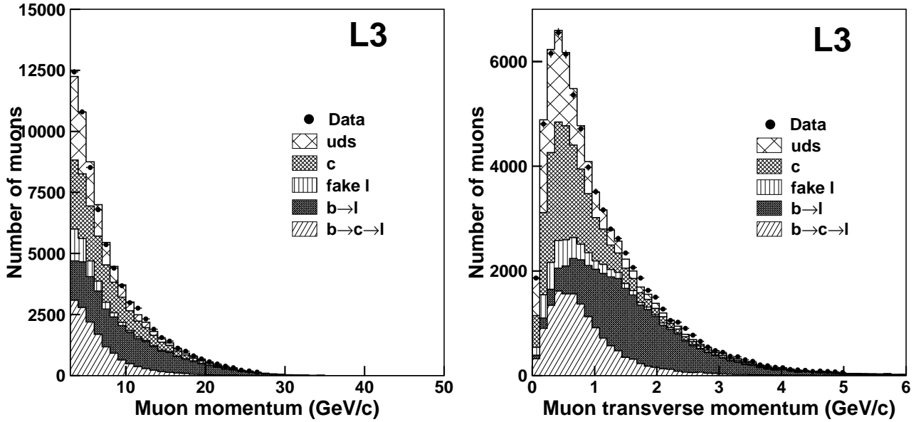
Figure 5.5: Muon momentum and transverse momentum spectra obtained by L3, together with expectations from simulation for the contributions from the various sources.
