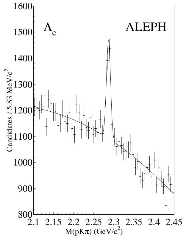
Figure 5.7: Mass spectra for D^0 \rightarrow K^- \pi^+ , D^+ \rightarrow K^- \pi^+ \pi^+ , D_s \rightarrow K^+ K^- \pi^+ and \Lambda_c^+ \rightarrow p K^- \pi^+ obtained by ALEPH [131].
