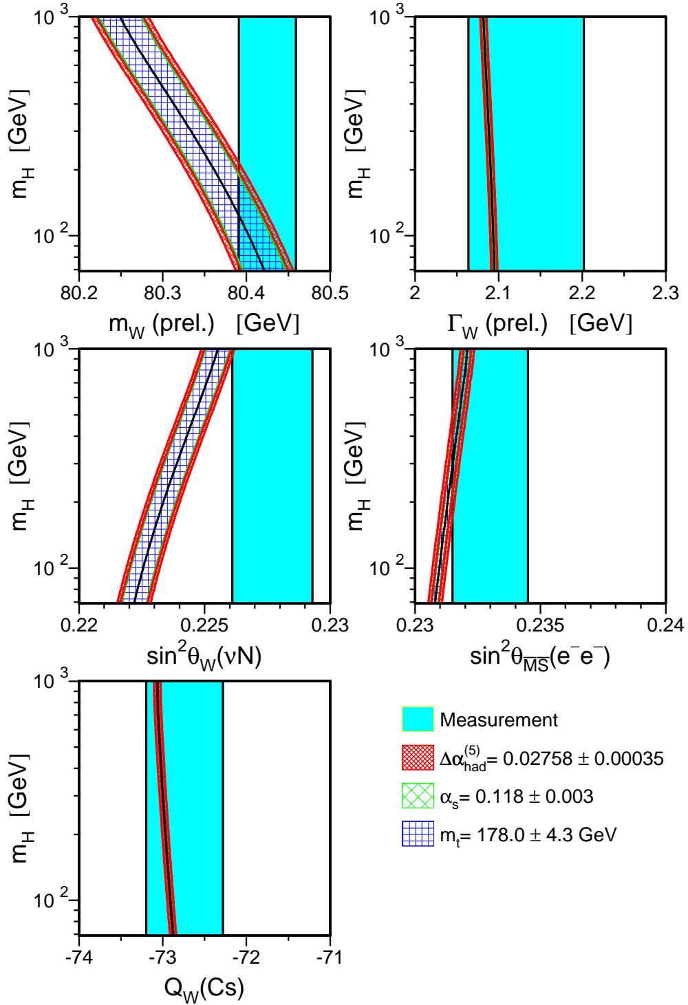
Figure 8.7: Comparison of the combined measurements of m_W and \Gamma_W , and the results from low Q^2 processes \sin^2 \theta_W (\nu N) , \sin^2 \theta_{\overline{\text{MS}}}(m_Z) (e^-e^-) and Q_W (APV) with the SM prediction as a function of the mass of the Higgs boson. The measurement with its uncertainty is shown as the vertical band. The width of the SM band arises due to the uncertainties in \Delta\alpha_{\text{had}}^{(5)}(m_Z^2) , \alpha_s(m_Z^2) and m_t in the ranges indicated. The total width of the band is the linear sum of these uncertainties. The direct measurements of m_W and \Gamma_W used here are preliminary.
