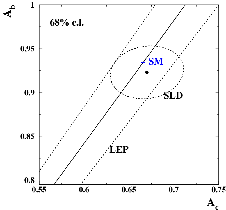
Figure 5.17: Contours in the \mathcal{A}_c - \mathcal{A}_b plane and ratios of forward-backward asymmetries from the SLD and LEP, corresponding to 68 % confidence levels assuming Gaussian systematic errors. The SM prediction for m_t = 178.0 \pm 4.3 \text{ GeV} , m_H = 300_{-186}^{+700} \text{ GeV} and \Delta\alpha_{\text{had}}^{(5)}(m_Z^2) = 0.02758 \pm 0.00035 is also shown.
