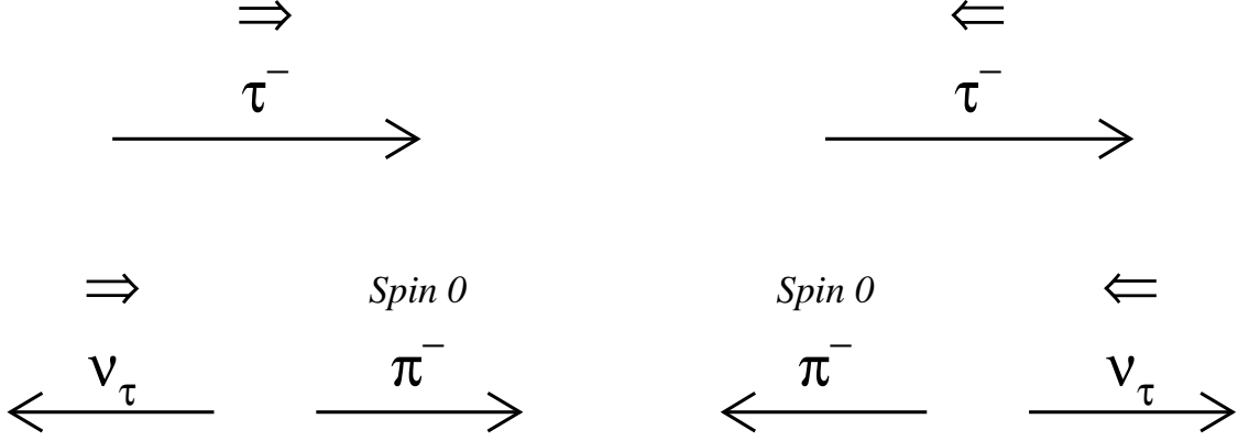
Figure 4.1: Decay configurations for two \tau helicity states for the decay \tau^- \rightarrow \pi^- \nu_\tau . The positive helicity configuration is on the left and the negative configuration is on the right. For each particle, the long arrow depicts the momentum direction while the short double arrow that of the spin. The lower pair of figures is depicted in the helicity rest frame of the parent \tau .
