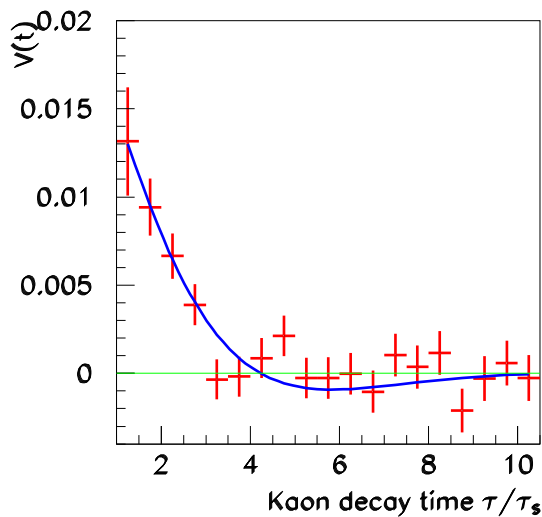
Figure 4: The experimental distribution V(t) (points with error bars, data summed over all kaon energies) and the function obtained from the fitted values for Re \lambda and Im \lambda for a mean kaon energy of 87 GeV.
