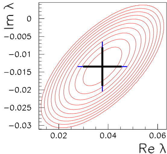
Figure 5: The fitted values of Re \lambda and Im \lambda in the complex plane with the contours for a \chi^2 of 1 to 10 above the minimum \chi^2 . The shorter error bars and the contours refer only to the statistical uncertainty while the longer error bars correspond to the total uncertainty.
