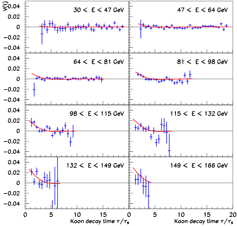
Figure 3: The experimental distribution V(t) (points with error bars) and the function obtained by a \chi^2 fit (smooth curve) in bins of time and energy. The \chi^2 per degree of freedom is 169.35/162=1.045 . The fit was made simultaneously over all energy bins, but is mainly constrained by the intermediate energy bins. The data were compensated for acceptance and trigger efficiency by applying Monte-Carlo corrections and by averaging over samples with opposite magnetic field in the spectrometer.
