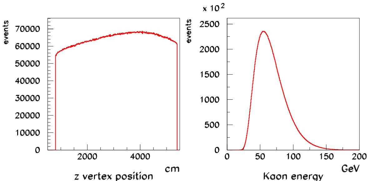
Figure 1: Position of the decay vertex along the beam line (left, measured from target position) and reconstructed K^0 energy (right) for the data sample of 19 million events.
