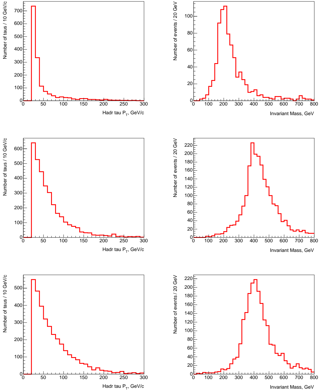
Figure 8: The \tau p_T distributions and the \tau - \tilde{\tau}_1 invariant-mass distributions for (a, b) benchmark scenario \epsilon , (c, d) benchmark scenario \zeta and (e, f) benchmark scenario \eta .
