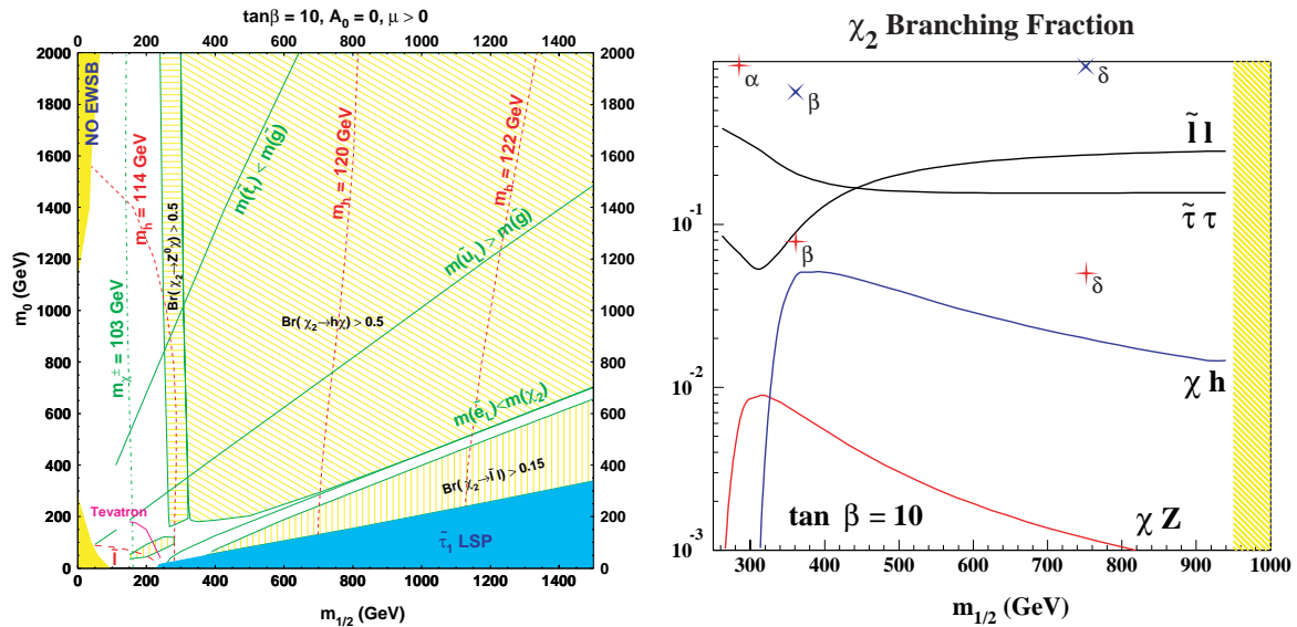
Figure 2: Left panel: Illustration of relevant aspects of the sparticle spectrum ordering and important decay modes in the (m_{1/2}, m_0) plane of the CMSSM for \tan\beta = 10, \mu > 0 and A_0 = 0 . Right panel: Decay modes of the second neutralino \chi_2 \rightarrow \chi Z (plus signs) and \chi h (crosses) in various NUHM and GDM benchmark scenarios, compared with the corresponding branching ratios along the the WMAP line for \tan\beta = 10 and \mu > 0 discussed in [9]. These plots were obtained with PYTHIA 6.215 [37] interfaced to ISASUGRA 7.69 [21].
