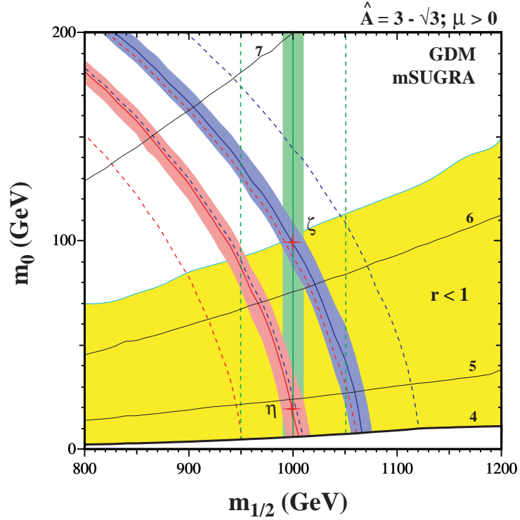
Figure 12: The potential impacts of prospective measurement errors of 1 % and 5 % for m_{\tilde{\tau}_1} (diagonal bands and lines) and m_{1/2} (vertical bands and lines) as constraints in the (m_{1/2}, m_0) plane for GDM models in the mSUGRA framework. The smaller errors would enable the benchmark scenarios \zeta and \eta to be distinguished, and the possible NLSP lifetime to be estimated. The thin solid lines are labeled by the logarithm of the NLSP lifetime in seconds.
