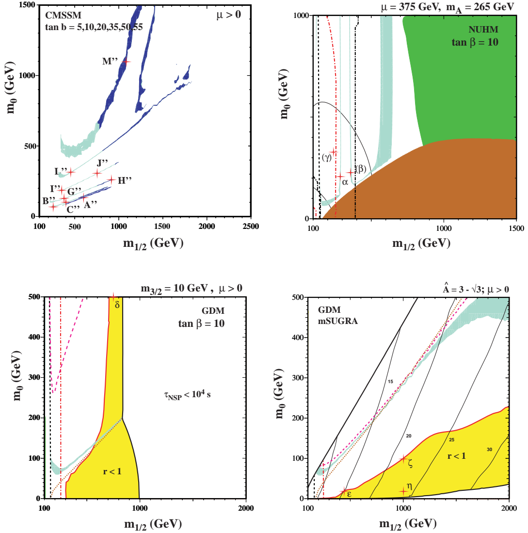
Figure 1: The allowed regions in the (m_{1/2}, m_0) planes for (a) the CMSSM with a neutralino LSP [light/dark (blue) shaded strips], (b) the NUHM with a neutralino LSP for \mu = 375 GeV and m_A = 265 GeV [light (blue) shaded strips], (c) the CMSSM with a gravitino LSP weighing 10 GeV, and (d) mSUGRA with a gravitino LSP [light (yellow) shaded regions labelled r < 1 ], for A \equiv \hat{A}m_0 : \hat{A} = 3 - \sqrt{3} . In each case, the proposed benchmark scenarios are indicated by (red) crosses. Panel (a) displays WMAP strips for \tan \beta = 5, 10, 20, 35, 50, 55 , panels (b, c) have \tan \beta = 10 , and in panel (d) \tan \beta is fixed by the electroweak vacuum conditions with the values indicated along the (solid black) contours.
