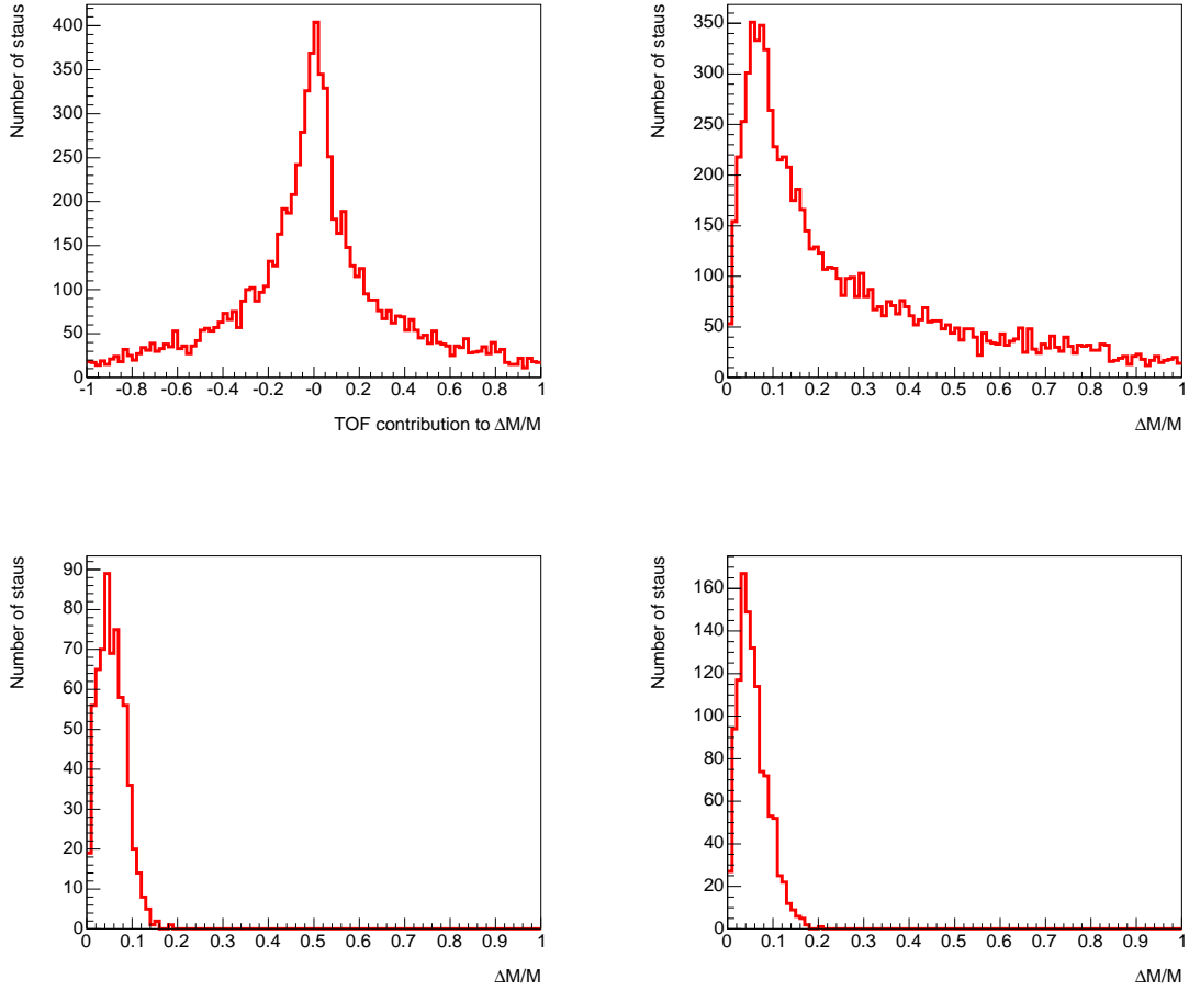
Figure 11: (a) The TOF contribution to the mass resolution \Delta M/M (6) in the stau NLSP mass measurement, (b) the full uncertainty \Delta M/M found for the complete event sample of benchmark point \epsilon , (c) \Delta M/M for the 10 % of events at point \epsilon with the lowest values of \beta\gamma^2 , and (d) the same distribution for point \zeta (the result for point \eta is very similar).
