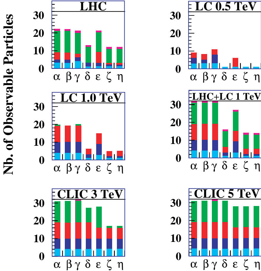
Figure 9: Summary of the numbers and types of MSSM particles that may be detected at various accelerators in the NUHM and GDM benchmark scenarios considered here. The gravitino may also be indirectly ‘observable’ at point \epsilon . We emphasize that these numbers are estimates that need to be validated by experimental simulations. As in [7, 9], we see that the capabilities of the LHC and of linear e^+e^- colliders are largely complementary. We re-emphasize that mass and coupling measurements at e^+e^- colliders are usually much cleaner and more precise than at the LHC, where, for example, it is not known how to distinguish the light squark flavours.
