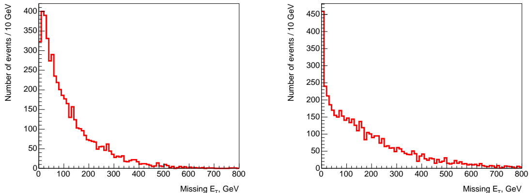
Figure 4: The missing E_T spectra in scenarios \epsilon and \zeta : that for point \eta is similar to the latter. These plots were obtained with PYTHIA [37] interfaced with ISASUGRA [21].
