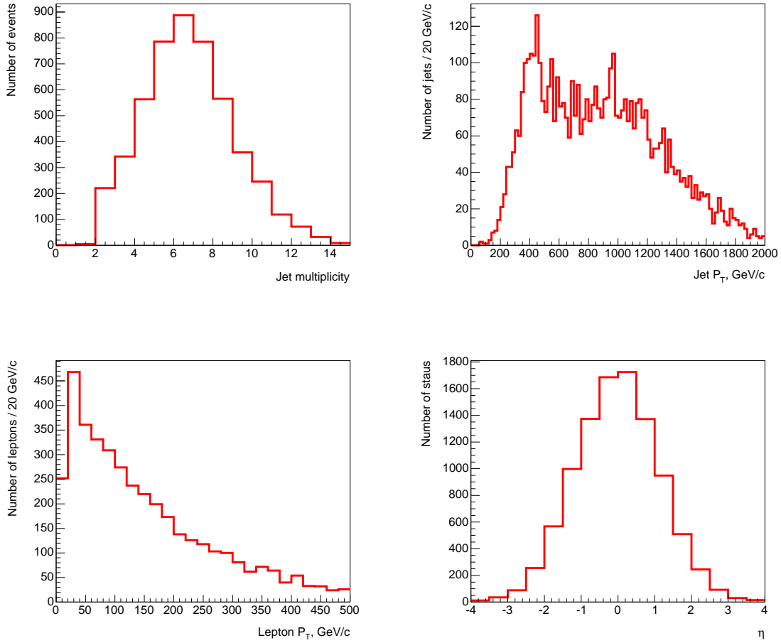
Figure 6: Kinematic distributions in events produced in the GDM benchmark scenario \zeta , as in Fig. 5.
