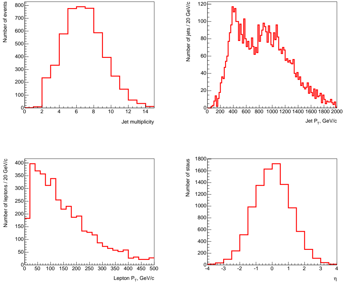
Figure 7: Kinematic distributions in events produced in the GDM benchmark scenario \eta , as in Fig. 5.
