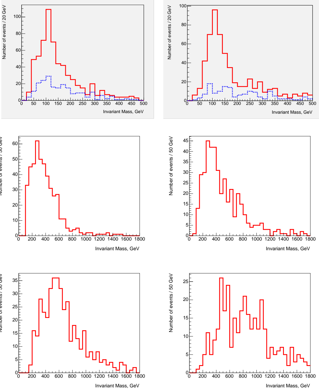
Figure 3: The signals from the lightest Higgs boson h in \chi_2 \rightarrow \chi h cascade decays in scenarios (a) \beta and (b) \delta , respectively, as found using PYTHIA [37] interfaced with ISASUGRA [21]. In each case, the solid line shows the sum of the supersymmetric signal and background, and the dashed line is the supersymmetric background alone. The Standard Model background is much smaller. The qh invariant mass distributions in scenarios (c) \beta and (d) \delta , respectively, each exhibit an end-point corresponding to \tilde{q}_R \rightarrow q\chi_2 cascade decays followed by \chi_2 \rightarrow \chi h . The q\tilde{q}h invariant mass distributions in scenarios (e) \beta and (f) \delta , respectively, each exhibit a feature corresponding to \tilde{g} \rightarrow \tilde{q}_R q and \tilde{q}_R \rightarrow q\chi_2 cascade decays followed by \chi_2 \rightarrow \chi h .
