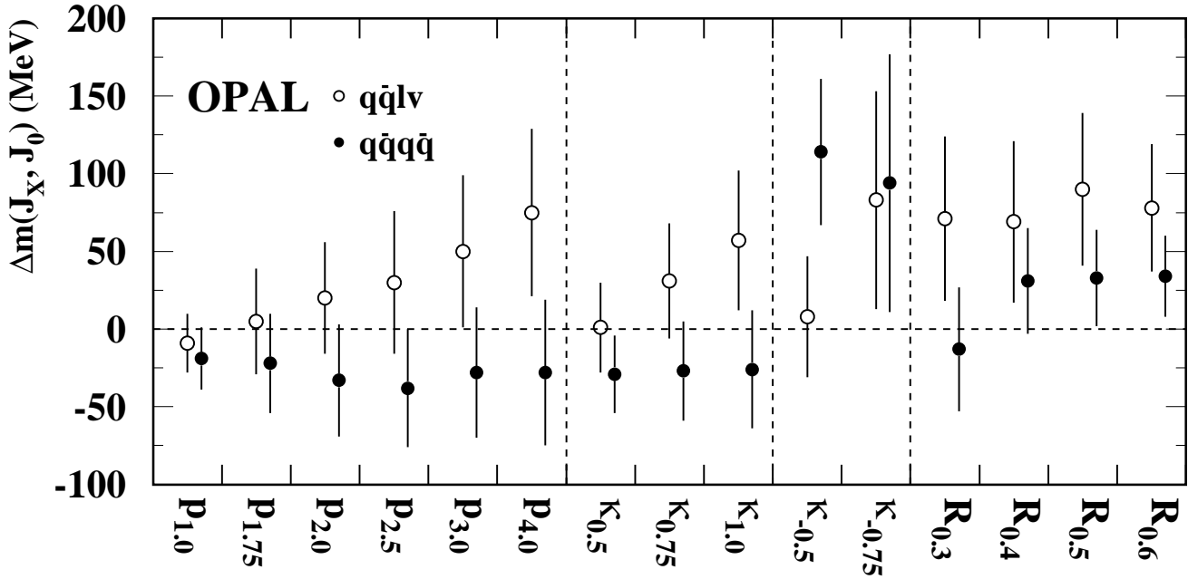
Figure 6: Differences in m_W measured using various jet direction reconstruction methods X and the J_0 reconstruction method, for both q\bar{q}l\nu and q\bar{q}q\bar{q} data in the convolution fit. The points are highly correlated; the errors are purely statistical and take into account the correlation between the result from each alternative direction reconstruction method and that from J_0 .
