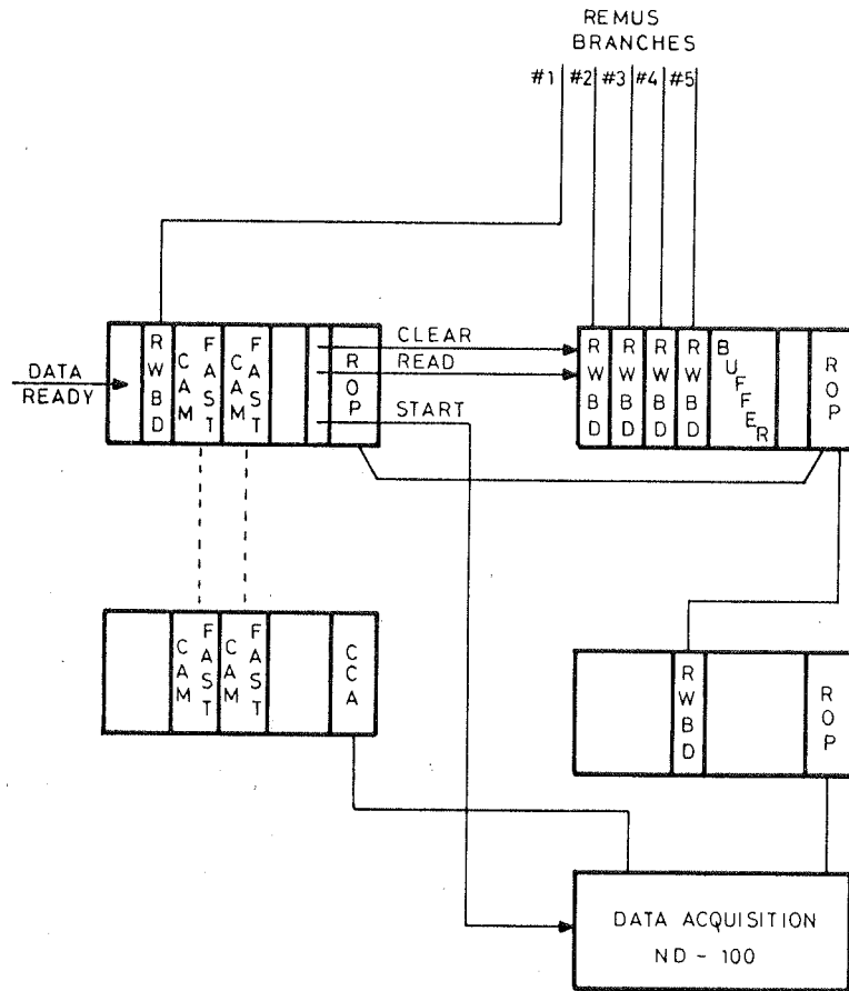
Fig. 5 Possible layout to use a double 168/E system on one branch of the UA-1 read-out
