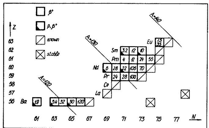
Fig. 3. Part of the isotopic chart showing the isotopes observed in the present investigation.
