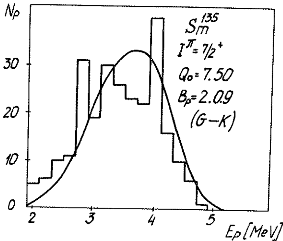
Fig. 7. The same as in fig. 6, for ^{135}\text{Sm} .
