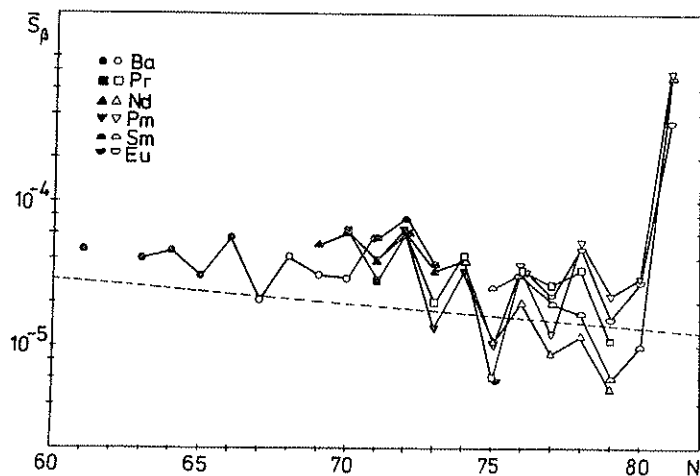
Fig. 4. Values of the averaged strength function ( \text{MeV}^{-1} \text{sec}^{-1} ) of the \beta^+ -EC-decay in the region of 61 N 81 for Ba, Pr, Nd, Pm, Sm and Eu isotopes.
