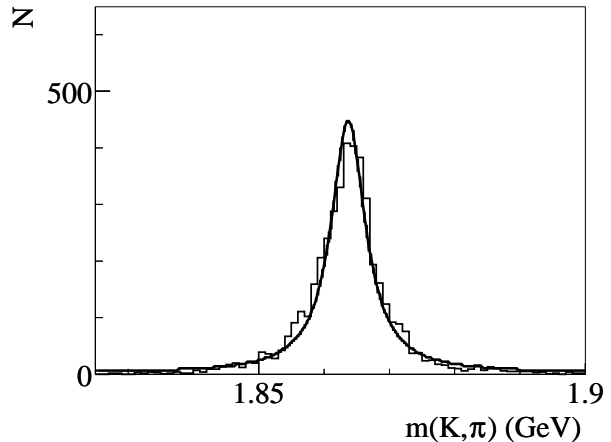
FIG. 3: Invariant mass distribution of simulated D^0 decays embedded in real data events. The full curve shows the Cauchy parameterization described in the text.
