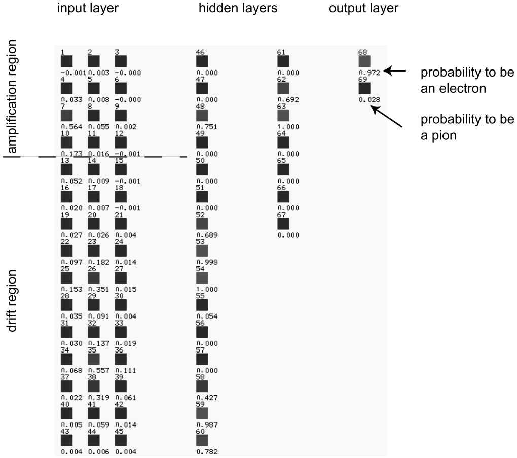
Fig. 3. NN topology for one TRD chamber. The left side is the input layer, in the middle the hidden layers and on the right side is the output layer. Note, that each neuron of a layer is connected with each neuron in the neighboring layers. For sake of clarity the connections are not drawn. The number below each neuron is the current excitation. Shown is a typical electron event. Three big clusters were generated (at neurons number 7, 26 and 35). The output layer displays the probabilities. In the present event the particle has been classified as an electron with a probability of 97.2 %.
