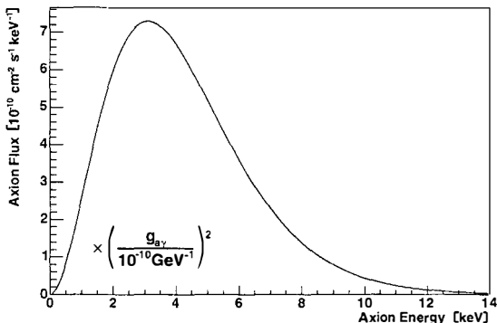
Figure 1: Axion flux spectrum at the Earth
