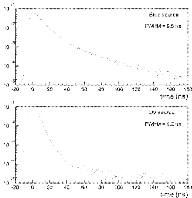
Fig. 4. Normalised distributions of photon arrival times measured in air with high statistics for the complete source sphere and with the full setup. Collimators are located between the source and the detector spheres.
