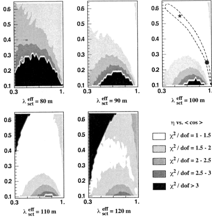
Fig. 15. \eta vs. \langle \cos \rangle for various slices in \lambda_{\text{set}}^{\text{eff}} . The various shades of grey separate equidistant regions with a difference of 0.5 in the normalised \chi^2 per degrees of freedom. The dashed line delimits the 1\sigma valley. The dot and the star correspond to the scattering parameters in table 4.
