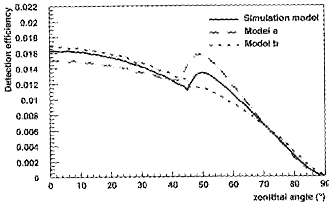
Fig. 17. Extreme models of the detector sphere angular efficiency (arbitrary units). The solid curve uses a parameterisation of the Moorhead and Tanner data [9] and is the model used in the simulation of the experimental setup. Model a (resp. model b) uses the thinnest (resp. the thickest) of the photocathodes together with the smallest (resp. the largest) complex refractive index.
