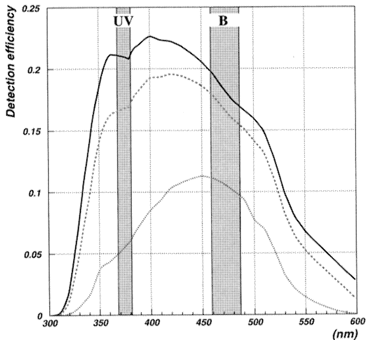
Fig. 1. Detection efficiency as a function of wavelength. The solid curve shows the PMT quantum efficiency and the absorption by the glass of the PMT, the optical gel and the protective glass sphere housing the PMT [19]. The dashed and dotted curves are calculated with a path length in water of 5 m and 30 m respectively, assuming a characteristic wavelength dependence of the water absorption length as given in [4]. The effect of scattering is not included. The bands labelled “B” and “UV” indicate the wavelengths at which measurements were undertaken at the ANTARES site.
