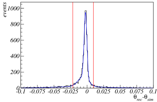
Fig. 6. Difference of reconstructed ( \theta_{rec} ) and emitted ( \theta_{sim} ) angle of the positrons. Angular scale is in radians.
