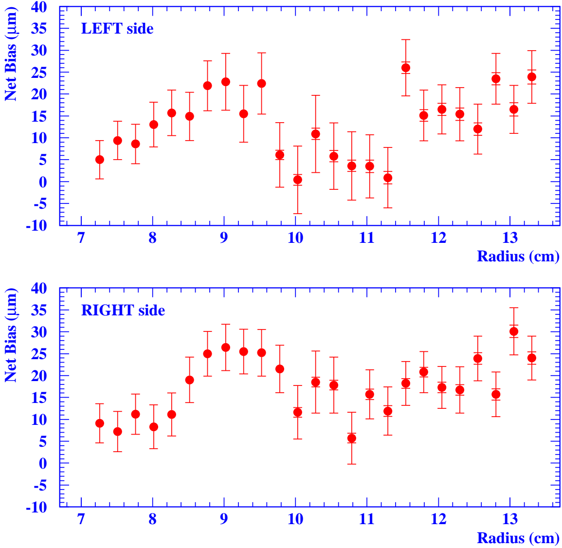
Figure 4: The total net bias \delta R (anchor) as a function of radius for the Left and the Right radial coordinate determined for the pad boundaries in the Si layer at 4 X_0 , for the combined 1993-94 data sample. The full error bars show the total error, the inner bars the statistical component.
