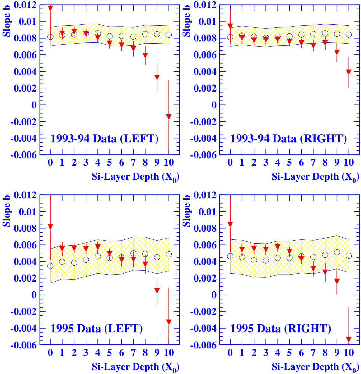
Figure 9: Fitted values of b as a function of the anchoring layer for homogeneous data subsamples. The open circles show results obtained from unanchored radial distributions, with the hatched band representing the (correlated) statistical error. The solid triangles show results from distributions corrected by anchoring, with the error bars representing only the systematic errors.
