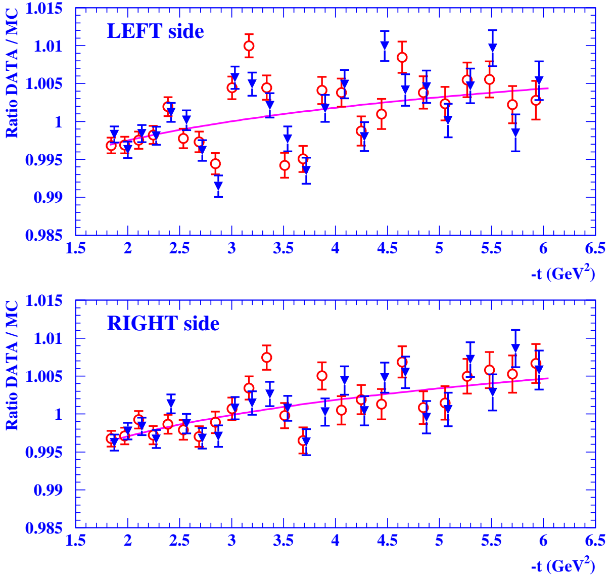
Figure 7: Ratios of numbers of data and Monte Carlo events (with \Delta\alpha set to zero) for the complete data statistics, for the Left and Right sides. Each point corresponds to a bin of one radial pad. The solid triangles show the data corrected with anchors in layer 4X_0 , the empty circles the unanchored data (slightly shifted horizontally for clarity), with statistical errors in both cases. The line shows the fit to the anchored data.
