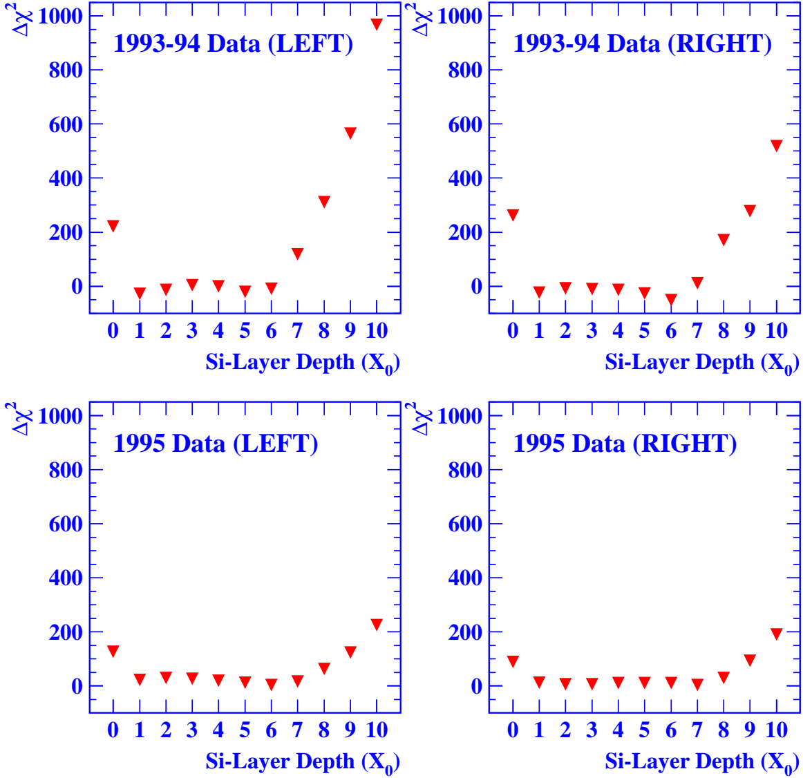
Figure 8: Difference in \chi^2 (for 22 degrees of freedom) between the fits of anchored and unanchored radial distributions as a function of the anchoring layer for homogeneous data subsamples. Only statistical errors are considered.
