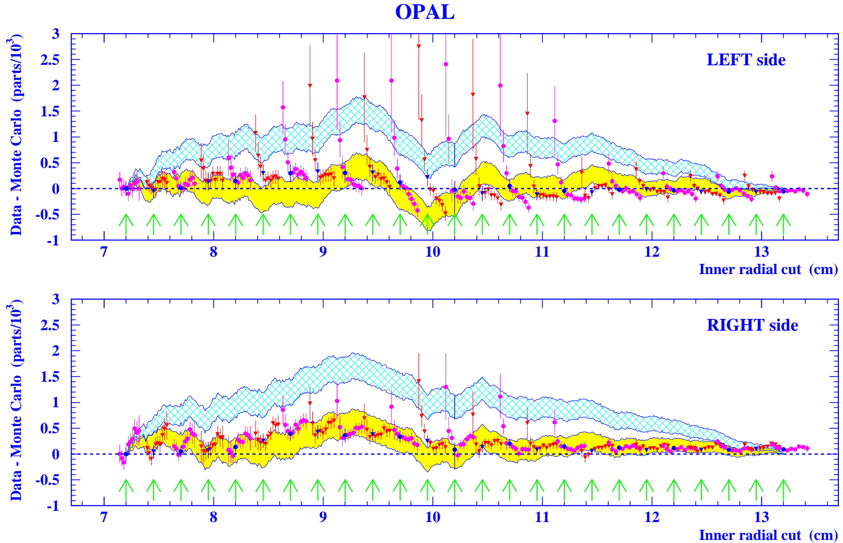
Figure 6: Study of the final reconstructed radial coordinate. The shaded band shows the relative change in acceptance between data and Monte Carlo as a function of the definition cut on the inner radius for the combined 1993-94 data sample. The width of the band shows the (highly correlated) statistical errors. The solid points show the acceptance variation determined by the anchoring procedure in Si layers from 1 X_0 to 10 X_0 , with the total errors shown. Triangles and circles designate even and odd rings of radial pads respectively. Within each group of points the arrow shows the location of the radial pad boundary in layer 7 X_0 , with deeper layers to the left and shallower layers to the right. The anchor at R = 7.2 cm is fixed to lie at zero. The hatched band shows the prediction for zero running ( \alpha(t) \equiv \alpha_0 ).
