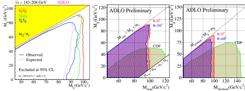
Figure 1. Left: excluded region (final) for pair produced sleptons decaying via \tilde{t} \rightarrow t + \chi_0 . The parameter space point is \mu = -200 GeV/c 2 , \tan(\beta) = 1.5 . Middle: excluded regions (preliminary) for pair produced stops decaying via \tilde{t} \rightarrow c\chi_0 . Right: excluded regions (preliminary) for pair produced sbottoms decaying via \tilde{b} \rightarrow b\chi_0 . Only squark masses above 50 GeV/c 2 are shown, since lower values have been excluded at LEP 1.
