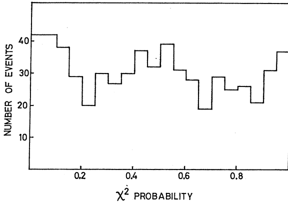
FIG. 5. \chi^2 probability distribution for a geometrical 5C fit constraining the \gamma rays to a common origin, applied to 4\gamma candidates.
