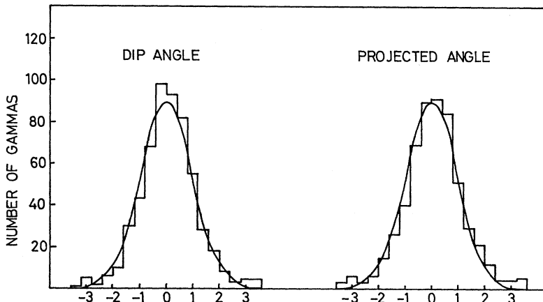
FIG. 4. Difference in (i) dip angle \delta and (ii) projected angle \phi between the known and measured directions of \gamma rays produced in visible interactions in the chamber liquid, in units of the calculated error in the difference. The curves show the distributions expected if the errors are correctly calculated, namely, Gaussians of unit variance.
