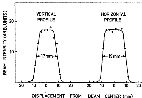
FIG. 2. Profile of the neutron component accompanying the K_L^0 beam, measured with a 1 \times 1 -mm finger counter just behind the bubble chamber.
