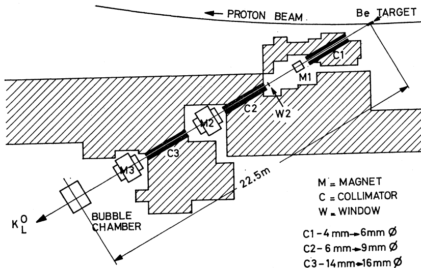
FIG. 1. Experimental layout.
