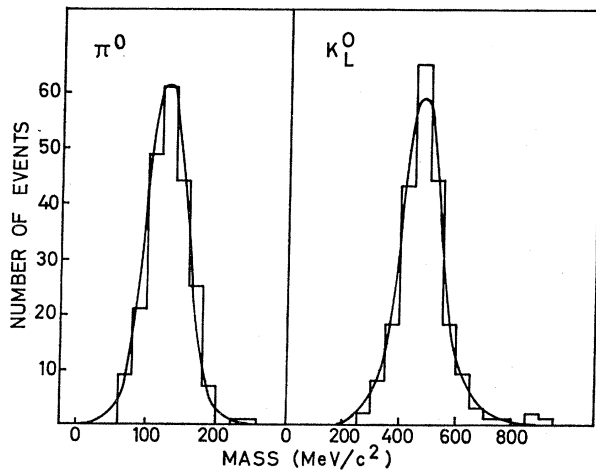
FIG. 6. Observed \pi^0 and K_L^0 mass distributions obtained by measuring \pi^0 \rightarrow 2\gamma and K_L^0 \rightarrow 3\pi^0 \rightarrow 6\gamma events with the techniques used to measure the 4\gamma candidates. The curves show the widths expected.
