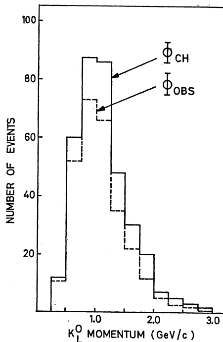
FIG. 3. Momentum distribution of the K_L^0 particles decaying in the fiducial region. \Phi_{\text{obs}} is the distribution directly observed. \Phi_{\text{ch}} is that obtained after correcting for losses.
