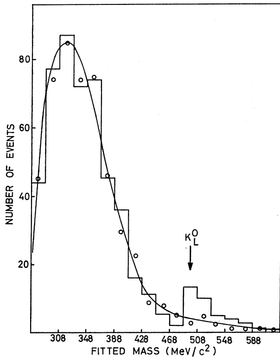
FIG. 8. Fitted mass distribution of observed 4\gamma candidates (histogram) and predicted background (points and curve).
