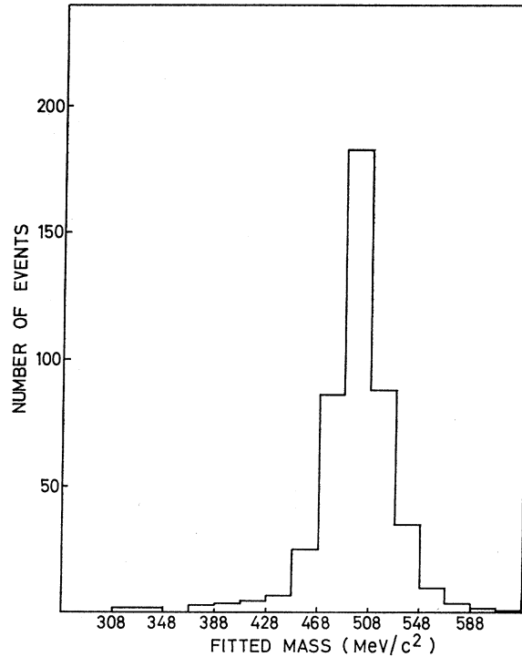
FIG. 9. Fitted mass distribution of Monte Carlo K_L^0 \rightarrow 2\pi^0 \rightarrow 4\gamma events.
