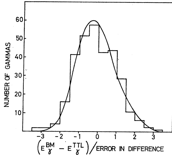
FIG. 7. Difference between TTL and BM energy values, for \gamma rays in 4\gamma candidates, in units of the error in the difference. The solid curve shows the distribution expected.
