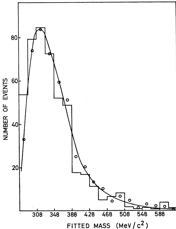
FIG. 10. Fitted mass distributions of artificial K_L^0 \rightarrow 3\pi^0 \rightarrow 4\gamma events generated by rejecting \gamma rays two at a time from (i) measured 6\gamma events (histogram) and (ii) Monte Carlo 6\gamma events (points and curve).
