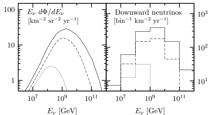
FIG. 3: Left: cosmogenic neutrino fluxes referred in the text as higher (solid), lower (dashed) and minimal (dotted). We plot the fluxes for one flavor \Phi = \phi_{\nu_\ell} + \phi_{\bar{\nu}_\ell} and assume that all flavors have the same frequency. Right: corresponding number of downward ( 0 \leq \theta_z < \pi/2 ) cosmogenic neutrinos of each flavor.
