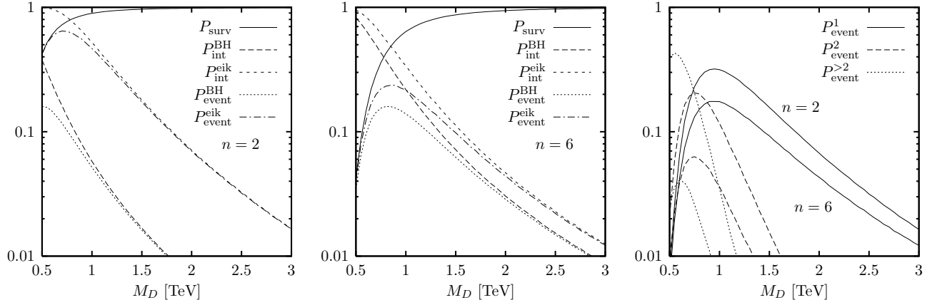
FIG. 4: The different probabilities defined in the text for a 10^{10} GeV neutrino reaching IceCube from \theta_z = 0 as a function of M_D for n = 2 and n = 6 .
