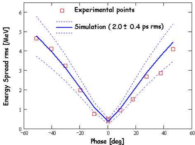
FIG. 15: Energy spread as a function of the RF phase shift for the accelerating structures and simulations for a bunch length of (2.0 \pm 0.4) ps rms.
