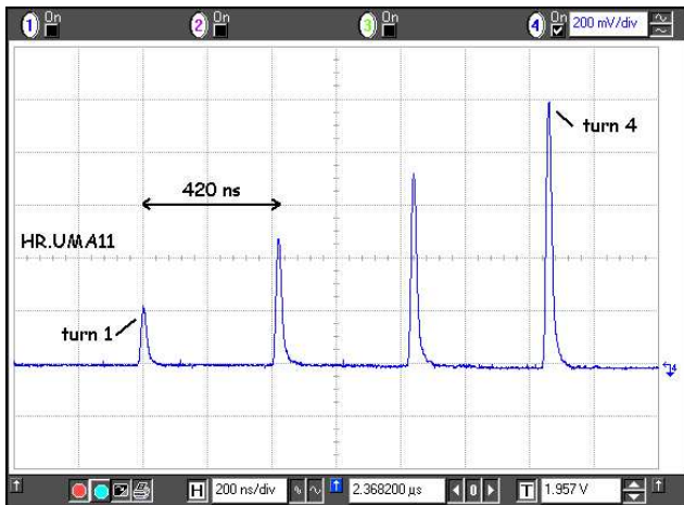
FIG. 19: Intensity signal of a beam position monitor in the ring for a bunch combination with a factor four.
