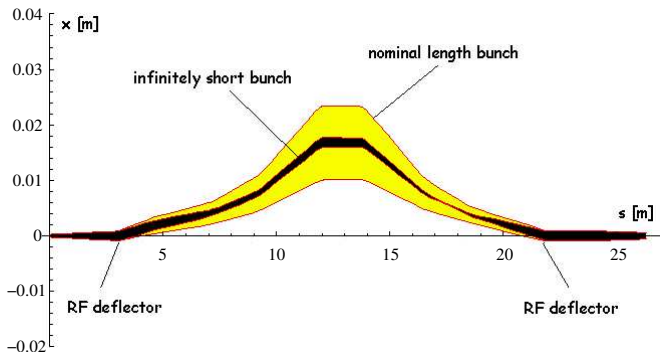
FIG. 5: Simulated beam envelopes of the bunches of Fig. 4 in the case of an infinitely short bunch and of a bunch length of 3 ps rms. Both bunches have a normalized rms emittance of 15 \pi mm mrad and are located at 2\pi/5 on the RF deflecting field.
