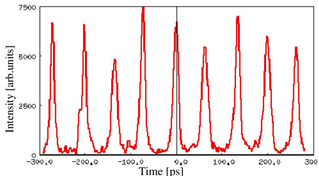
FIG. 22: Longitudinal intensity profiles for a multiplication factor five.
