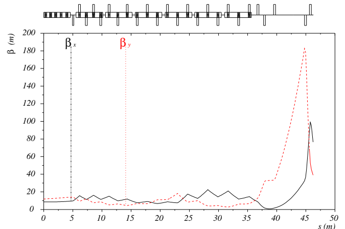
FIG. 6: Design optics of the linac and the matching section between the exit of the bunching system and the injection line. The horizontal (solid line) and vertical (dashed line) \beta -functions are shown.
