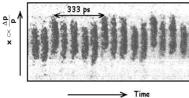
FIG. 23: Streak camera image of a combined beam (factor five), showing bunch-to-bunch variations in transverse position. The dispersion function at the observation point is |D_x| \simeq 3 m. A periodicity corresponding to the combination factor is clearly visible.
