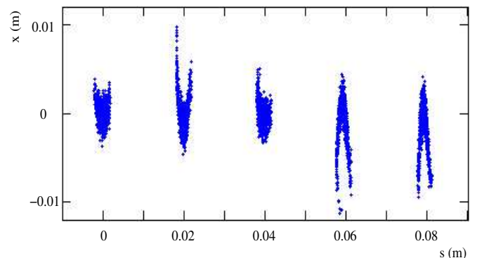
FIG. 9: Horizontal transverse versus longitudinal position for a combination factor five in the combiner ring with realistic energy spread for the injected bunches.
