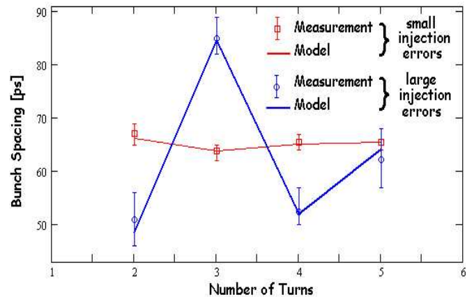
FIG. 27: Bunch spacing variations after the combination of two pulses as a function of the number of turns for large (circles) and small (squares) injection errors. The solid curves correspond to the model predictions in both cases.
