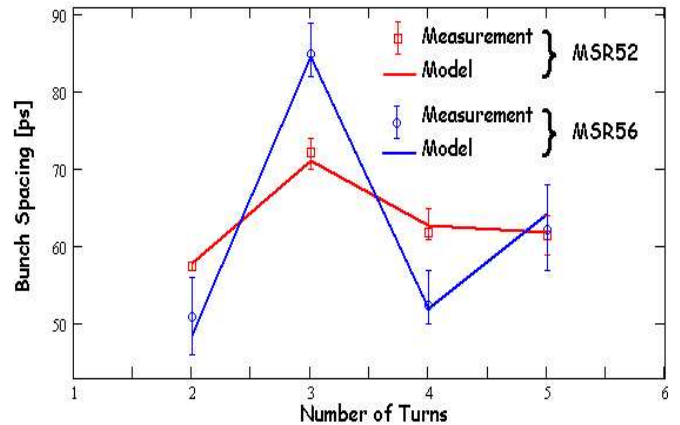
FIG. 26: Bunch spacing variations after the combination of two pulses as a function of the number of turns observed from two different synchrotron light ports (squares and circles, respectively) in the case of large injection errors. The solid curves correspond to the model predictions in both cases.
