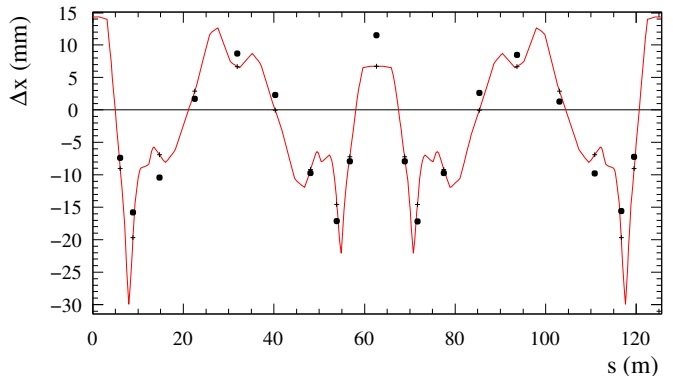
FIG. 14: Measured horizontal closed orbit difference (black points) for a change in frequency from 19.089942 to 19.083229 MHz. The solid line corresponds to the expected closed orbit difference, proportional to the dispersion calculated from a model with the measured magnet currents.
