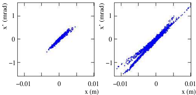
FIG. 10: Horizontal phase space at the extraction point after five turns. The left plot corresponds to the case of a perfectly uniform kick at injection, the right plot is obtained when using RF deflectors for a bunch combination factor of five.
