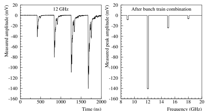
FIG. 29: Bunch frequency monitor signals at 12 GHz, while a bunch train combination with a factor four occurs (left) and amplitude of the four harmonics of interest measured on the oscilloscope at the end of the bunch frequency multiplication (right).
