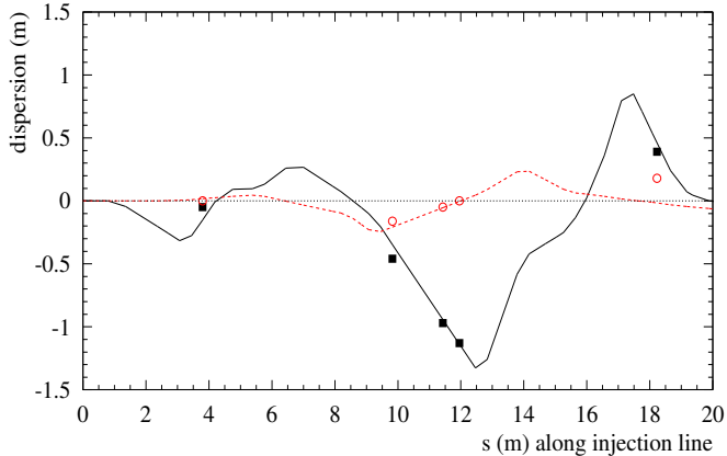
FIG. 12: Dispersion measurements in the injection line. The full squares are the experimental points in the horizontal plane and the solid curve is given by the model for the corresponding current settings. The open circles and the dashed line are measurements and expectations from the MAD model in the vertical plane, respectively.
