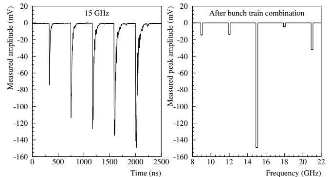
FIG. 28: Bunch frequency monitor signals at 15 GHz, while a bunch train combination with a factor five occurs (left) and amplitude of the five harmonics of interest measured on the oscilloscope at the end of the bunch frequency multiplication (right).
