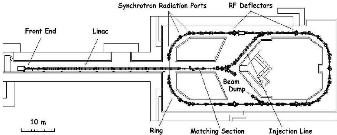
FIG. 1: General layout of the CTF3 Preliminary Phase.
