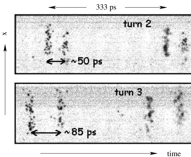
FIG. 25: Turn-to-turn bunch spacing variations during the combination of two pulses with injection errors. The bunch spacing changes from 50 ps at the second turn (top) to 85 ps at the third turn (bottom).
