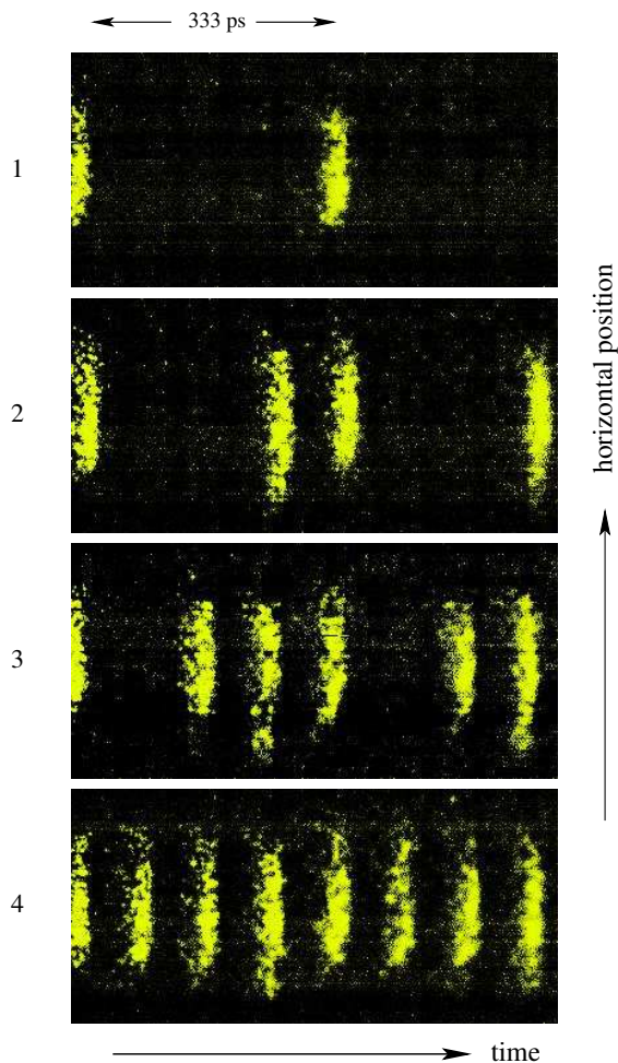
FIG. 20: Bunch train combination with a factor four, as observed with a streak camera. The horizontal axis represents time, the vertical axis corresponds to the horizontal position. The images from top to bottom are taken over four consecutive turns.
