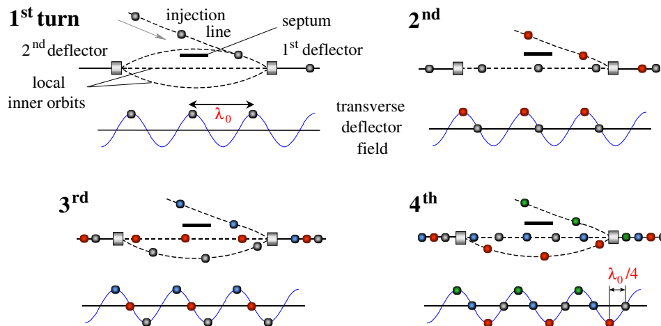
FIG. 2: Bunch train combination by injection with RF deflectors for a multiplication factor four. The images show the injection region of the ring for four successive turns of injected bunches and the corresponding bunch distribution on the RF field of the deflectors.
