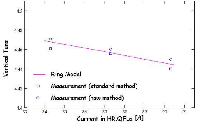
FIG. 13: Vertical tune measurements in the ring in accumulation mode as a function of the current in one quadrupole family and comparison between two methods and the MAD model. For clarity, the error bars on the measurement points ( \pm 0.01 ) are omitted.
