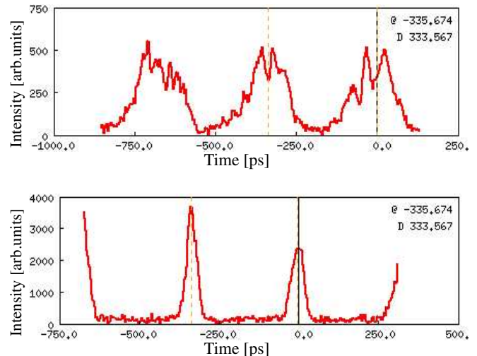
FIG. 16: Longitudinal intensity profile as measured with the streak camera. The top profile is taken during the second turn for the non-isochronous optics. The bottom image shows the distribution in the 60 th turn for the isochronous optics.
