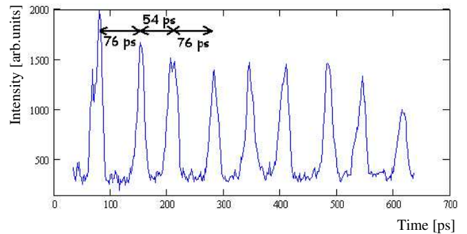
FIG. 24: Longitudinal intensity profile for bunch train combination of factor five showing bunch spacing variations. Here, the correct bunch spacing should be 333/5 \simeq 67 ps.
