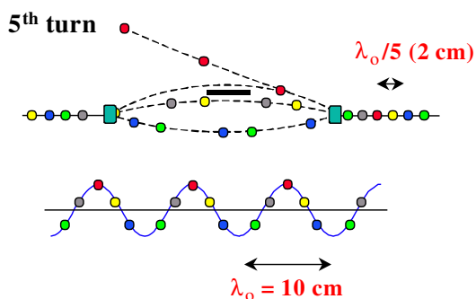
FIG. 3: Fifth passage of the first injected bunch train in the injection region for a combination with a multiplication factor of five.
