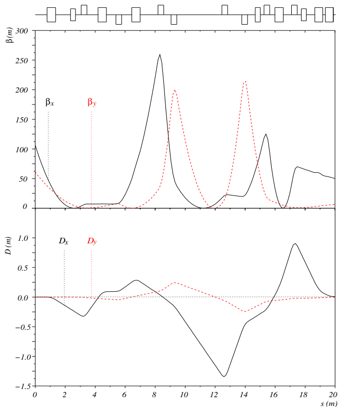
FIG. 7: Design optics of the injection line. The horizontal (solid line) and vertical (dashed line) \beta -functions are shown on the top graph, design dispersion functions for the horizontal (solid line) and vertical (dashed line) plane on the bottom.
