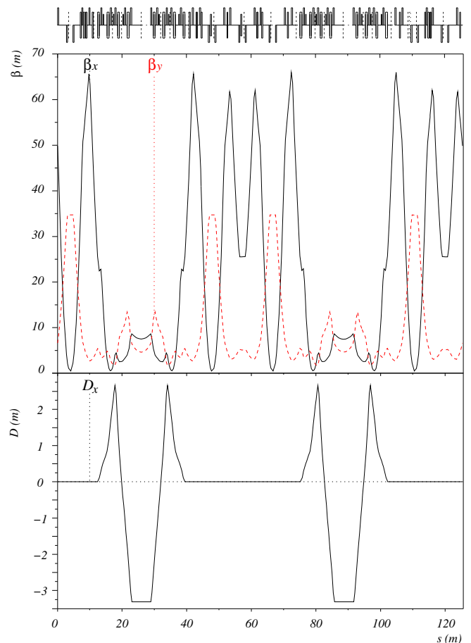
FIG. 8: Design optics of the isochronous combiner ring starting from the injection point. The top graph shows the horizontal (solid line) and vertical (dashed line) \beta -functions, the bottom graph the design horizontal dispersion function. The vertical dispersion is zero.
