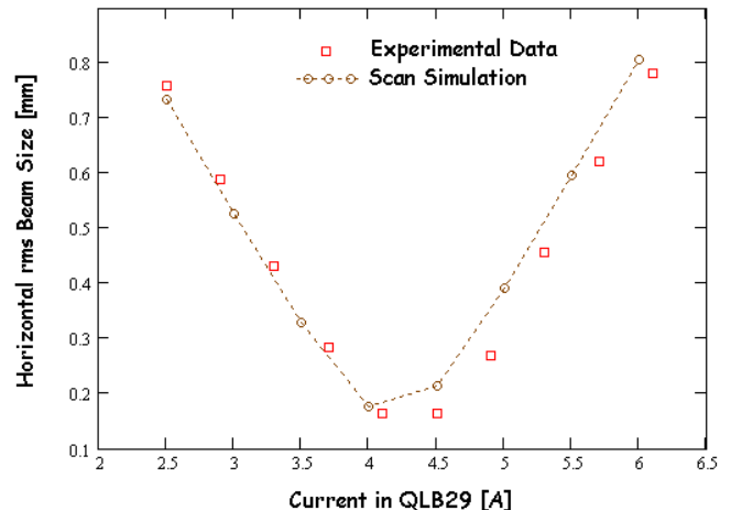
FIG. 11: Transverse beam size measured by a Wire Beam Scanner as a function of the quadrupole current. The measured data points (squares) are compared to a simulated scan (circles) that is based on the initial Twiss parameters back-propagated from a downstream measurement.
