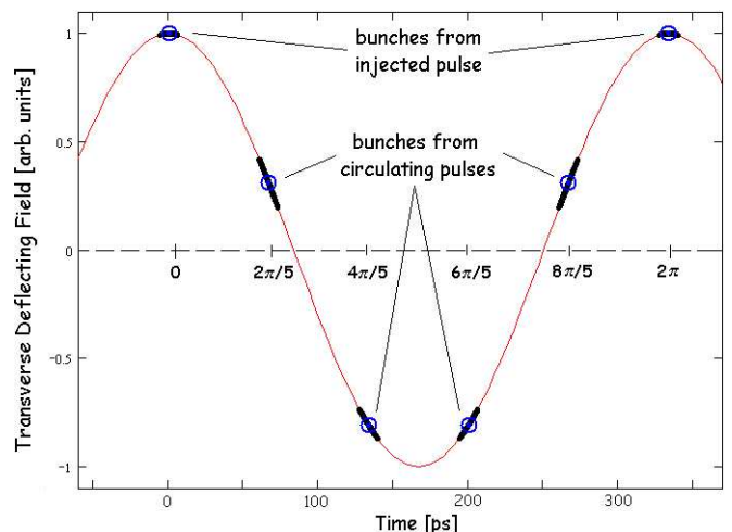
FIG. 4: Kick amplitude for injected and circulating bunches for a combination factor five. The longitudinal extension corresponds to \pm 2\sigma for a bunch with a Gaussian distribution with 3 ps rms bunch length. The circles indicate the centres of the bunches.
