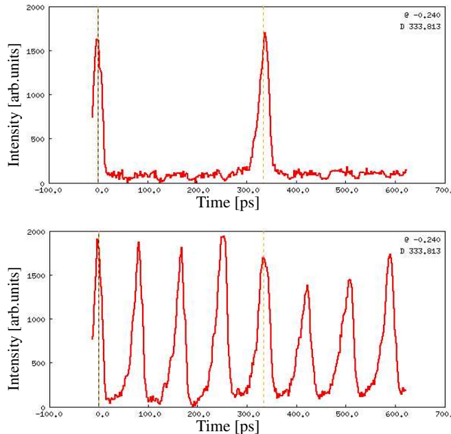
FIG. 21: Longitudinal intensity profiles for a multiplication factor four. The two images correspond to the injection of one and four bunch trains, respectively. Amplitude variations are due to bunch current variations already present in the linac.
