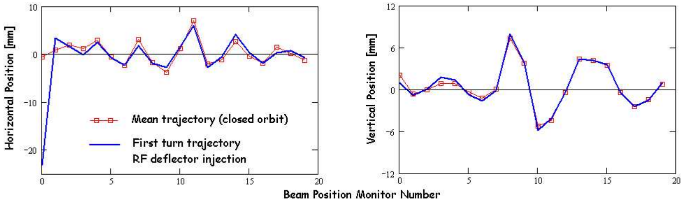
FIG. 18: Reference closed orbit and first turn trajectory in the isochronous ring in both planes. The reading in the first BPM shows the beam position at injection, before the deflector kick.
