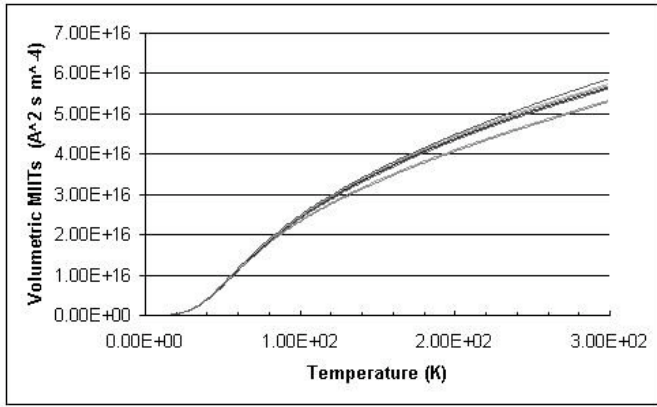
Fig. 2. Comparison of MIITs curve computations relying on different data sources for Cu and G10. The volume fractions of the conductor components are calculated according to the NED reference design, i.e. : Cu=52%, Nb 3 Sn=10%, Ta=4%, Bronze=18%, G10=16%.
