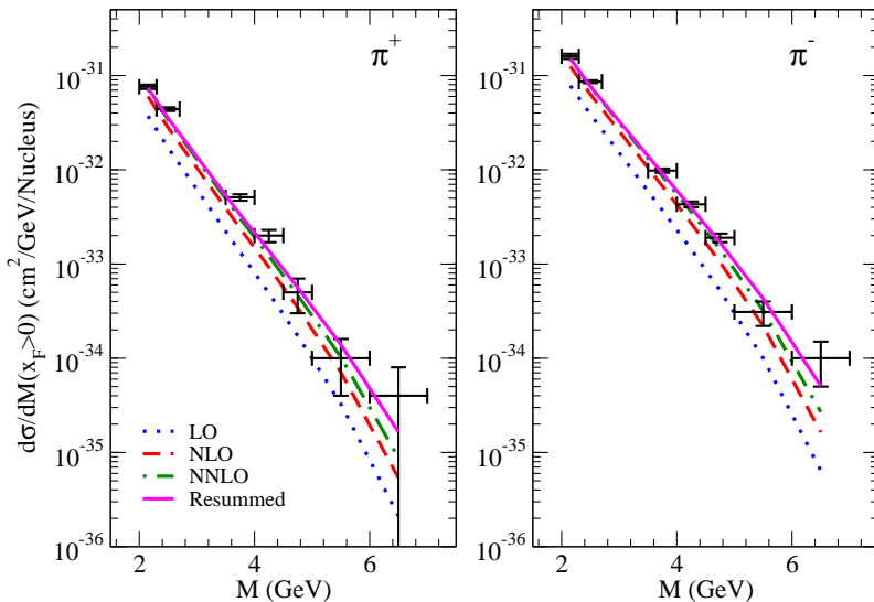
Figure 5: Comparison of LO, NLO, NNLO and resummed results to the WA39 data [45] for Drell-Yan dimuon production in \pi^\pm W scattering.
