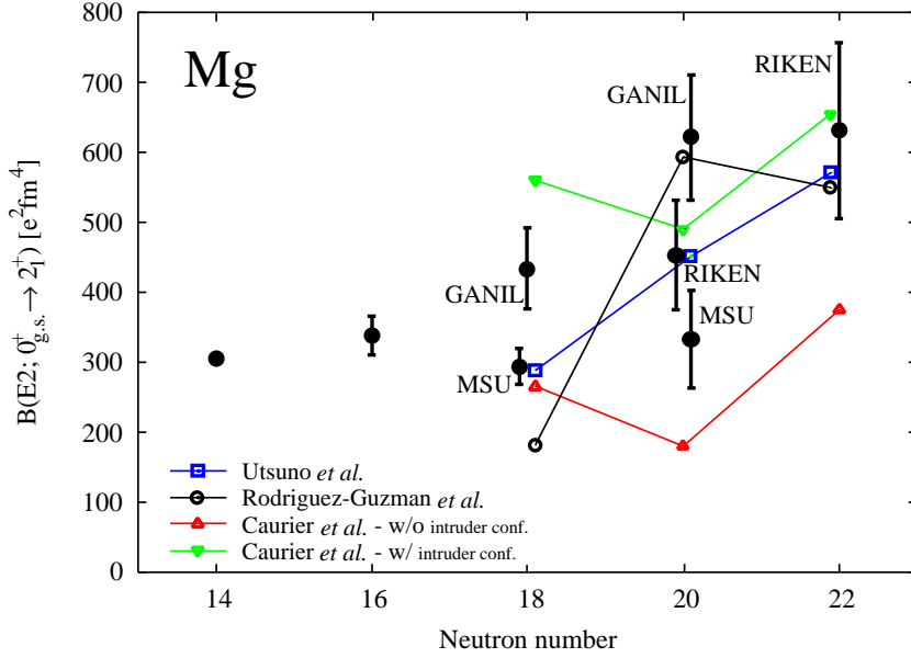
Figure 1. B(E2; 0_{gs}^+ \rightarrow 2_1^+) values for the neutron-rich even-even magnesium isotopes. The references are: Utsuno-[18], Rodriguez-Guzman-[19], Caurier-[20], GANIL-[16], MSU-[15], RIKEN-[14,17]. See text for details.
