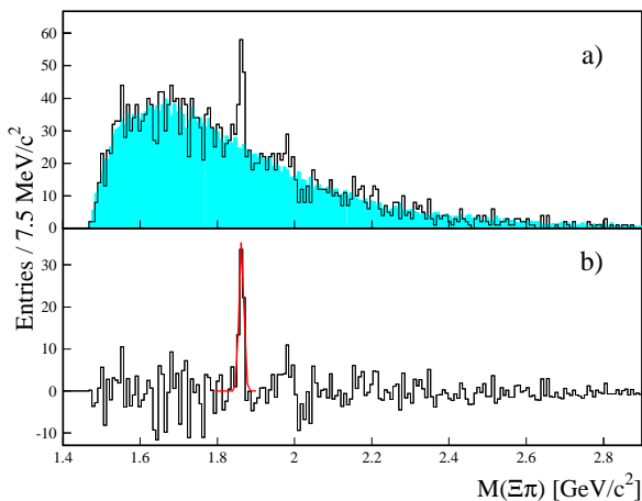
FIG. 3: (Color online) (a) The sum of the \Xi^-\pi^- , \Xi^-\pi^+ , \Xi^+\pi^- and \Xi^+\pi^+ invariant mass spectra. The shaded histogram shows the normalised mixed-event background. (b) Background subtracted spectrum with the Gaussian fit to the peak.
