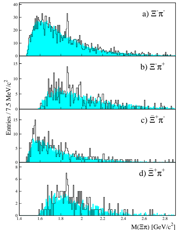
FIG. 2: (Color online) Invariant mass spectra after selection cuts for \Xi^-\pi^- (a), \Xi^-\pi^+ (b), \Xi^+\pi^- (note that the \Xi(1530)^0 state is also visible) (c), and \Xi^+\pi^+ (d). The shaded histograms are the normalised mixed-event backgrounds.
